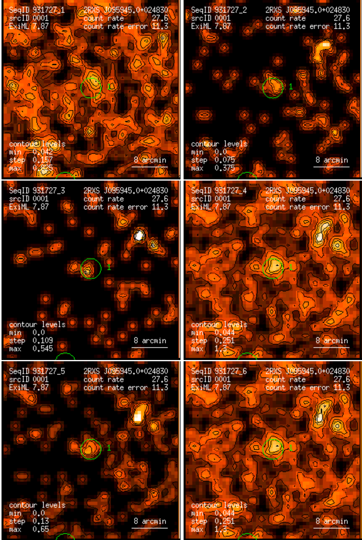
Figure 1: RASS 931727: detection 0001: band rate images, Gaussian filter: (1) PSPC channels 11 – 41, (2) 52 – 90, (3) 91 – 201, (4) 11 – 235, (5) 52 – 201, (6) 11 – 201. Broad band rates in counts/ks. Band rate contour levels in counts/ks/arcmin 2 .
