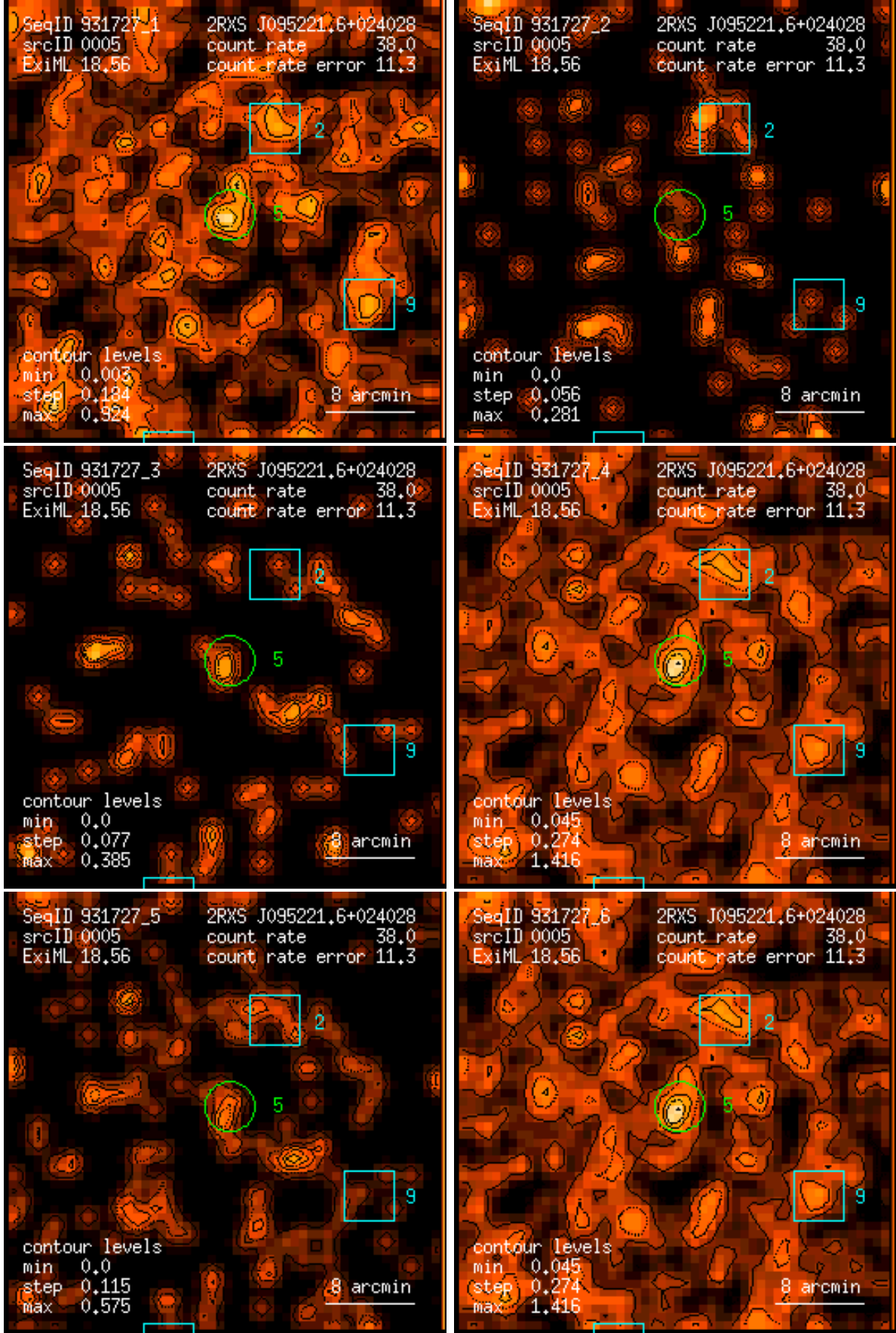
Figure 5: RASS 931727: detection 0005: band rate images, Gaussian filter: (1) PSPC channels 11 – 41, (2) 52 – 90, (3) 91 – 201, (4) 11 – 235, (5) 52 – 201, (6) 11 – 201. Broad band rates in counts/ks. Band rate contour levels in counts/ks/arcmin 2 .
