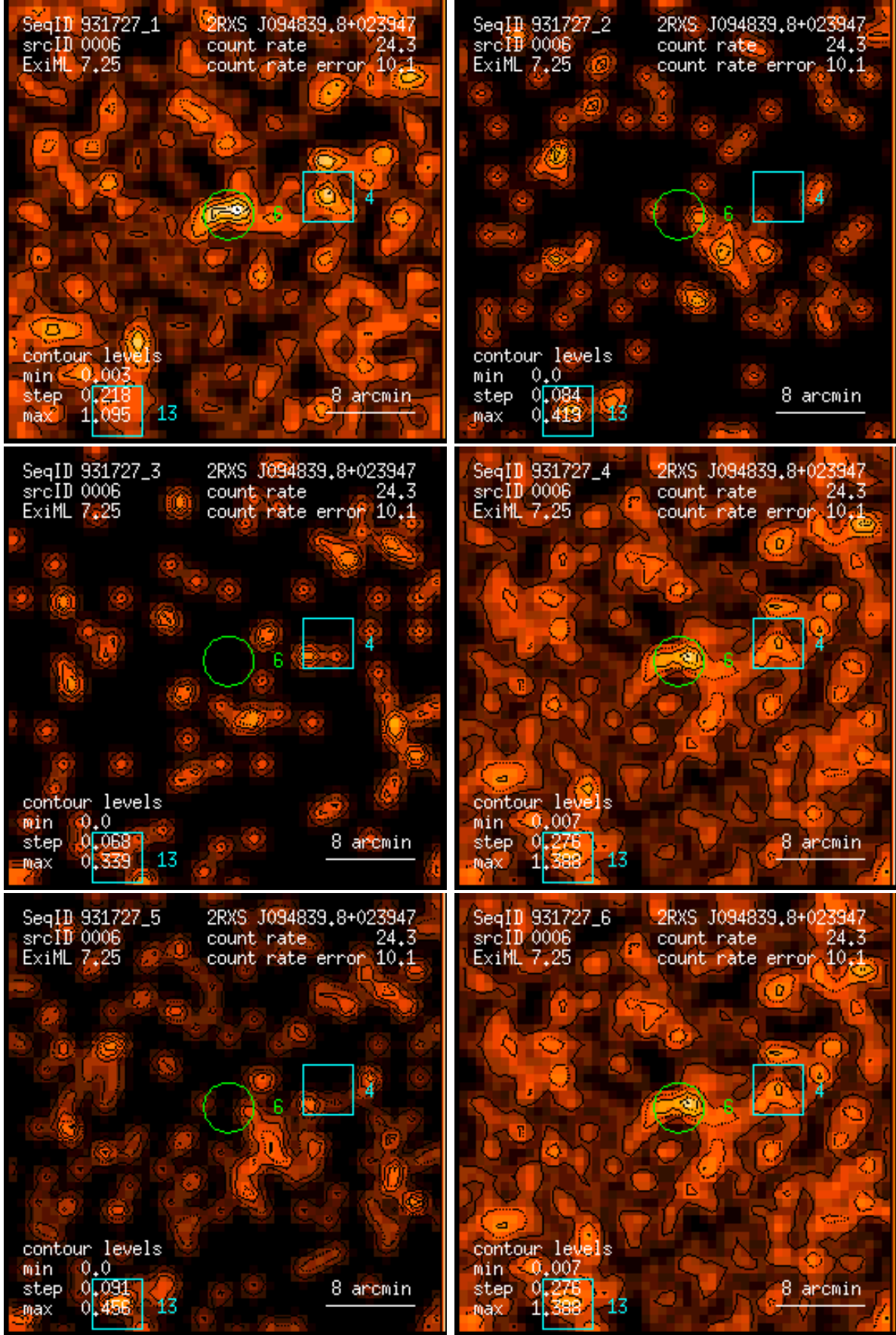
Figure 6: RASS 931727: detection 0006: band rate images, Gaussian filter: (1) PSPC channels 11 – 41, (2) 52 – 90, (3) 91 – 201, (4) 11 – 235, (5) 52 – 201, (6) 11 – 201. Broad band rates in counts/ks. Band rate contour levels in counts/ks/arcmin 2 .
