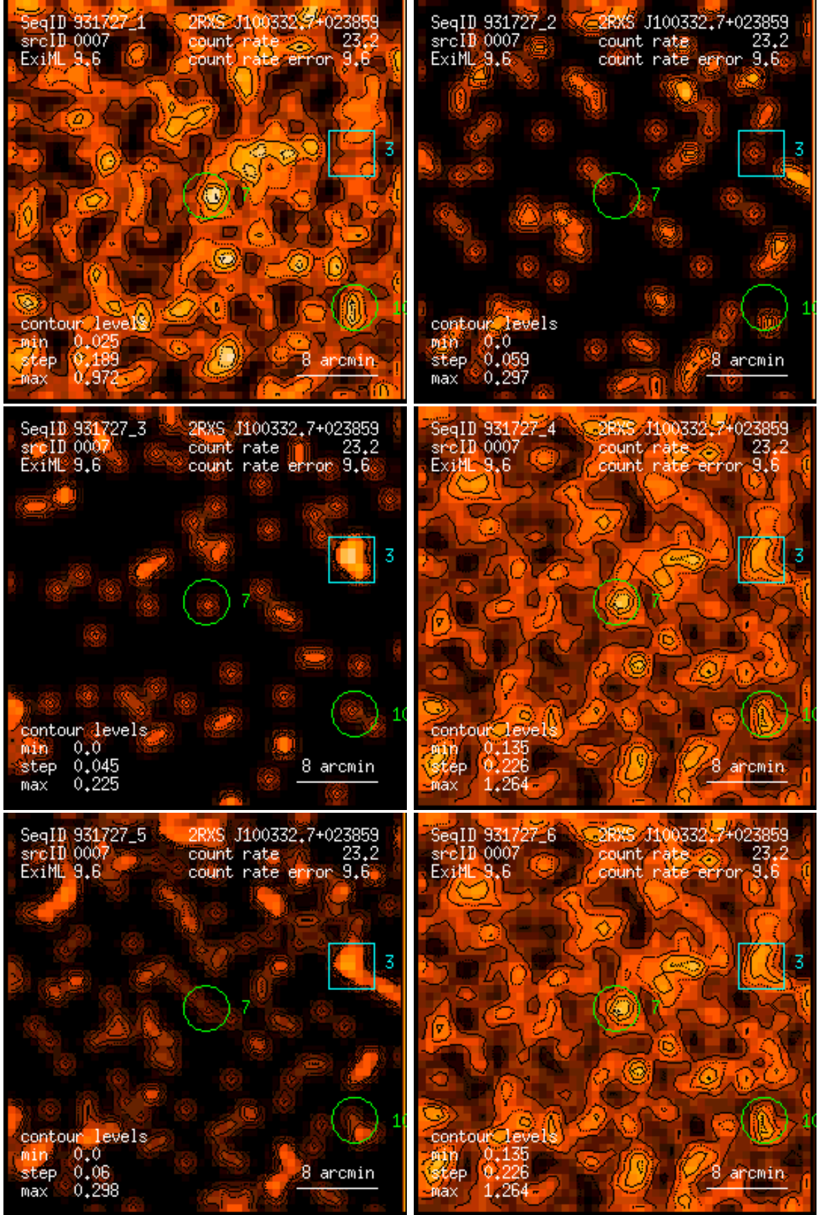
Figure 7: RASS 931727: detection 0007: band rate images, Gaussian filter: (1) PSPC channels 11 – 41, (2) 52 – 90, (3) 91 – 201, (4) 11 – 235, (5) 52 – 201, (6) 11 – 201. Broad band rates in counts/ks. Band rate contour levels in counts/ks/arcmin 2 .
