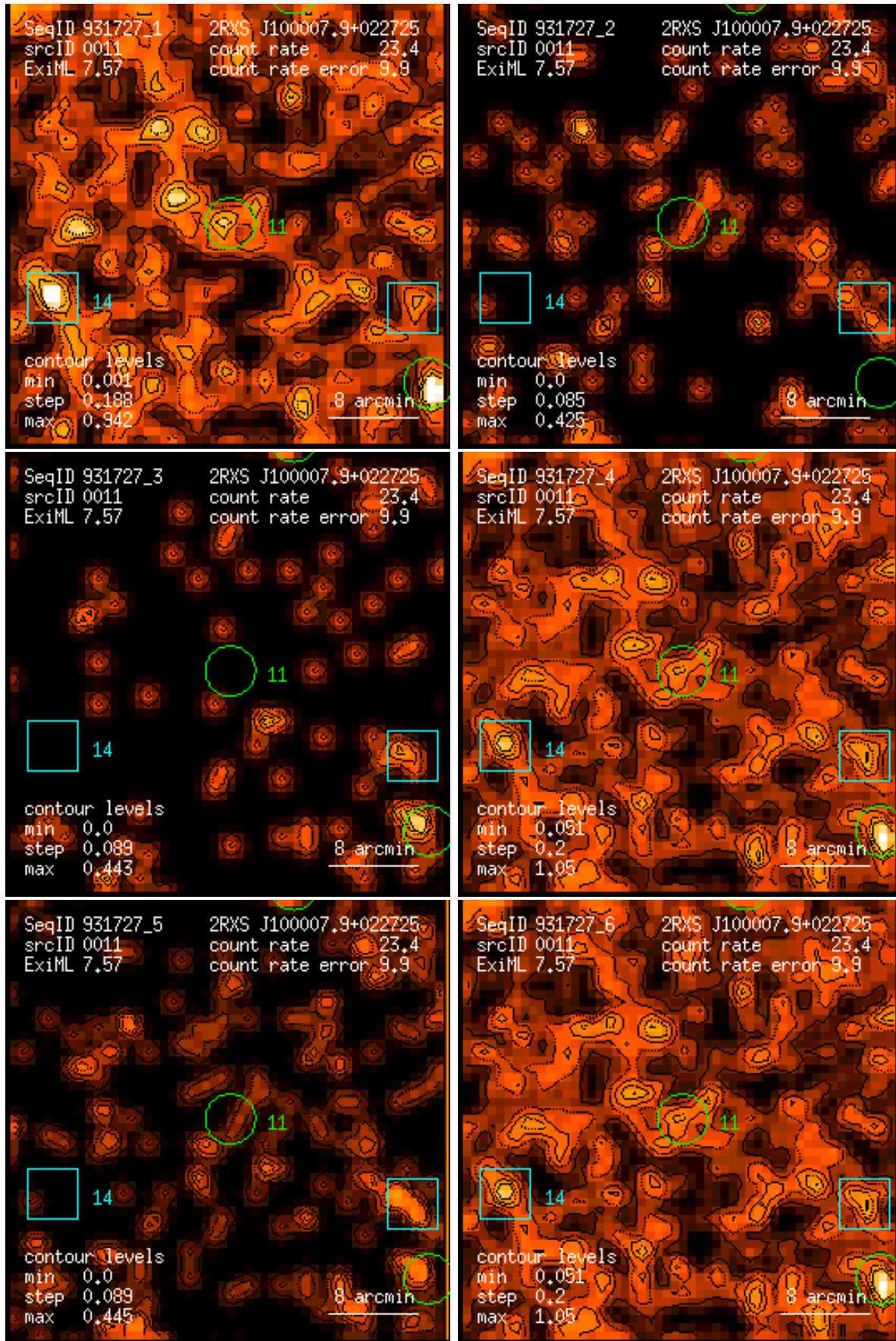
Figure 11: RASS 931727: detection 0011: band rate images, Gaussian filter: (1) PSPC channels 11 – 41, (2) 52 – 90, (3) 91 – 201, (4) 11 – 235, (5) 52 – 201, (6) 11 – 201. Broad band rates in counts/ks. Band rate contour levels in counts/ks/arcmin 2 .
