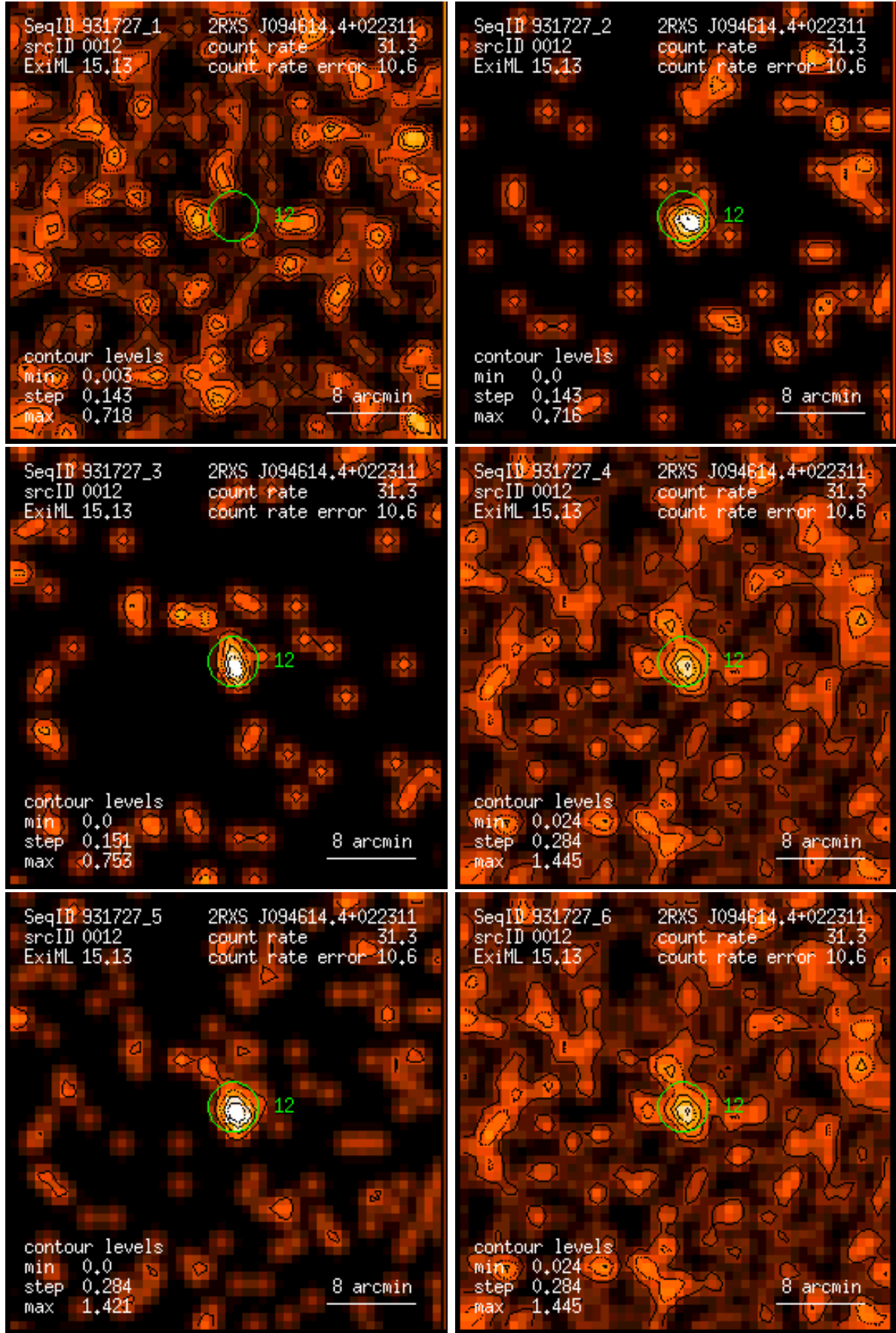
Figure 12: RASS 931727: detection 0012: band rate images, Gaussian filter: (1) PSPC channels 11 – 41, (2) 52 – 90, (3) 91 – 201, (4) 11 – 235, (5) 52 – 201, (6) 11 – 201. Broad band rates in counts/ks. Band rate contour levels in counts/ks/arcmin 2 .
