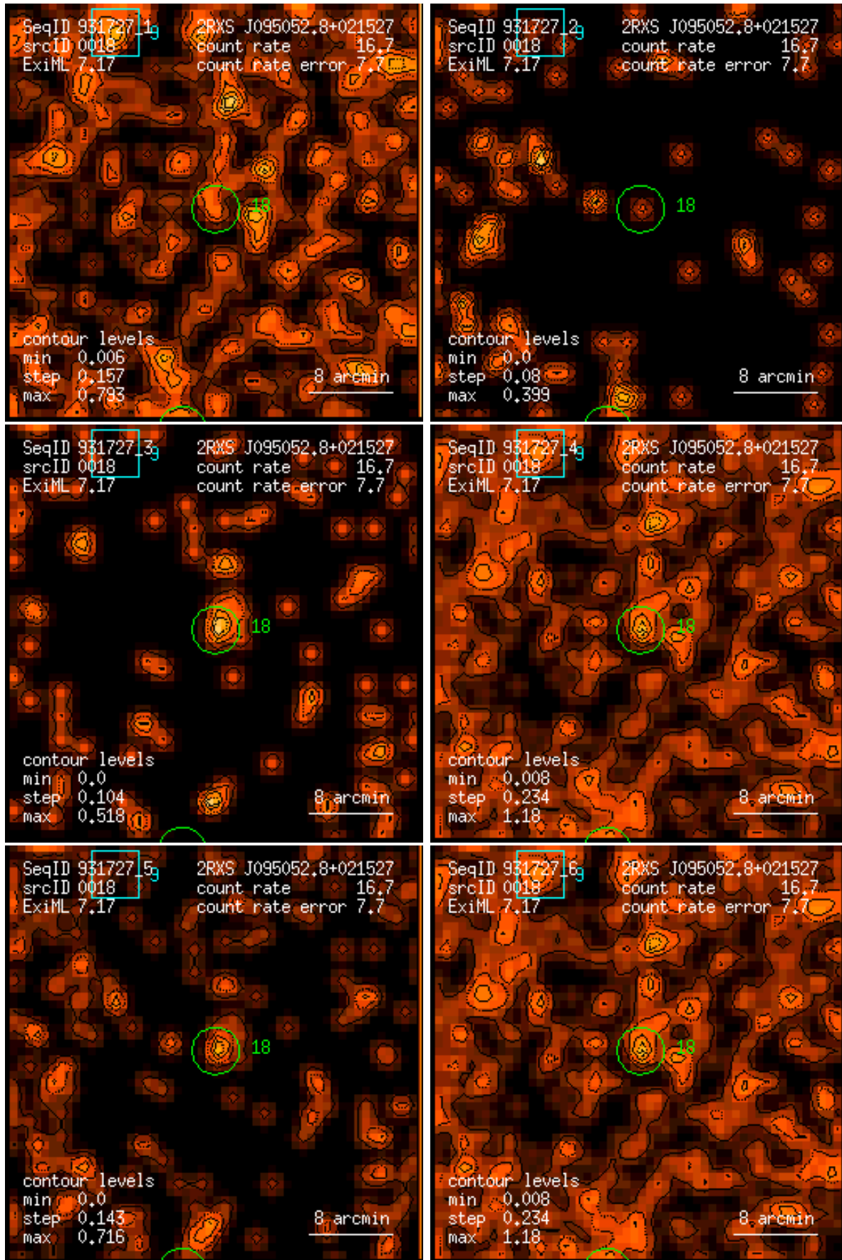
Figure 18: RASS 931727: detection 0018: band rate images, Gaussian filter: (1) PSPC channels 11 – 41, (2) 52 – 90, (3) 91 – 201, (4) 11 – 235, (5) 52 – 201, (6) 11 – 201. Broad band rates in counts/ks. Band rate contour levels in counts/ks/arcmin 2 .
