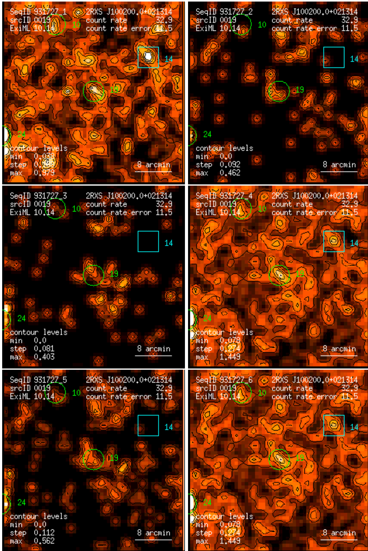
Figure 19: RASS 931727: detection 0019: band rate images, Gaussian filter: (1) PSPC channels 11 – 41, (2) 52 – 90, (3) 91 – 201, (4) 11 – 235, (5) 52 – 201, (6) 11 – 201. Broad band rates in counts/ks. Band rate contour levels in counts/ks/arcmin 2 .
