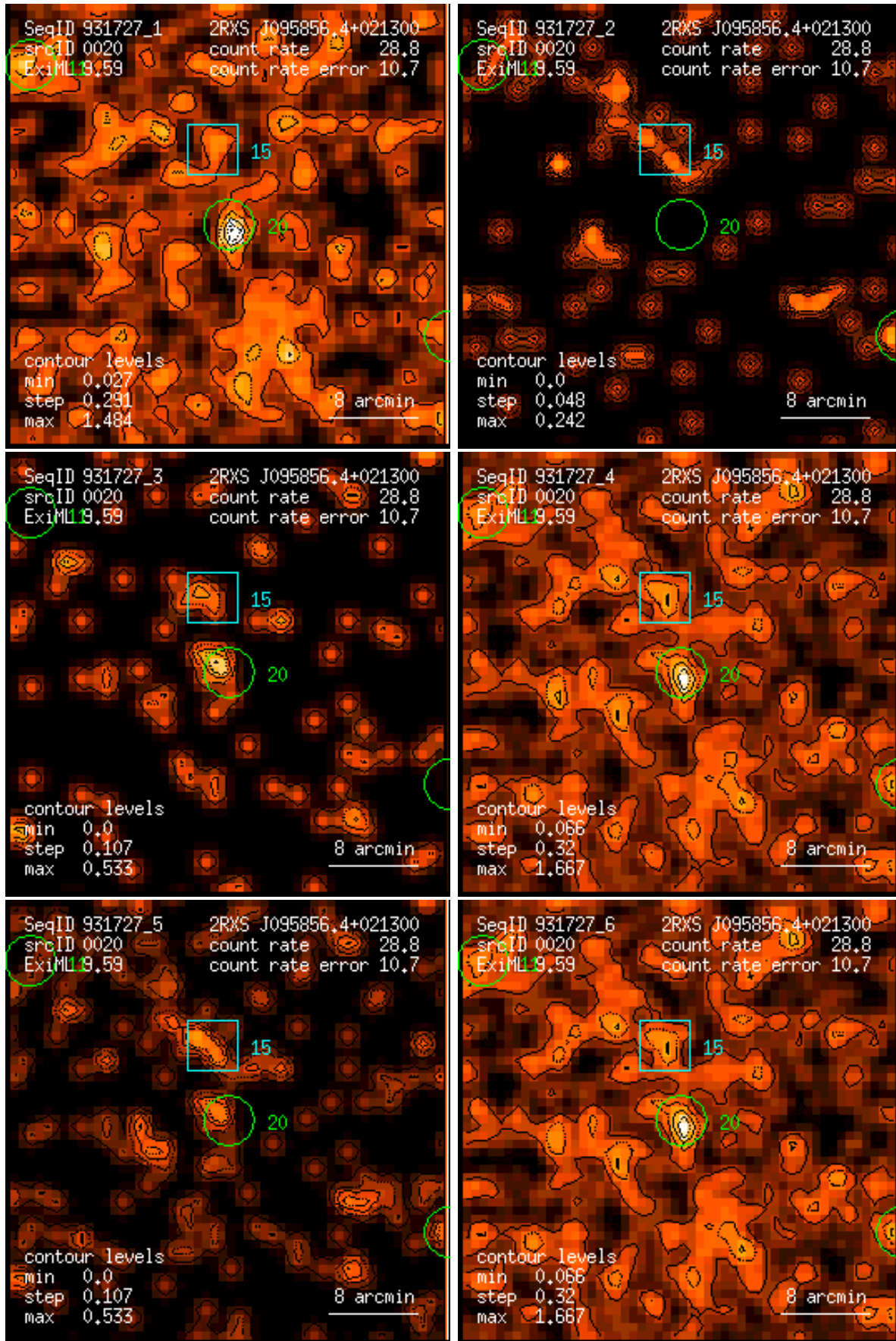
Figure 20: RASS 931727: detection 0020: band rate images, Gaussian filter: (1) PSPC channels 11 – 41, (2) 52 – 90, (3) 91 – 201, (4) 11 – 235, (5) 52 – 201, (6) 11 – 201. Broad band rates in counts/ks. Band rate contour levels in counts/ks/arcmin 2 .
