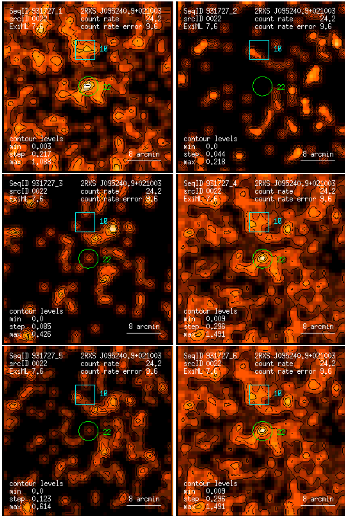
Figure 22: RASS 931727: detection 0022: band rate images, Gaussian filter: (1) PSPC channels 11 – 41, (2) 52 – 90, (3) 91 – 201, (4) 11 – 235, (5) 52 – 201, (6) 11 – 201. Broad band rates in counts/ks. Band rate contour levels in counts/ks/arcmin 2 .
