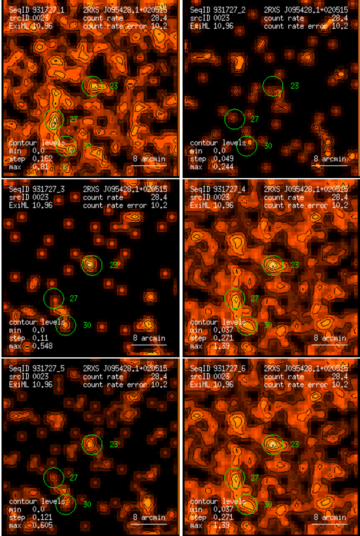
Figure 23: RASS 931727: detection 0023: band rate images, Gaussian filter: (1) PSPC channels 11 – 41, (2) 52 – 90, (3) 91 – 201, (4) 11 – 235, (5) 52 – 201, (6) 11 – 201. Broad band rates in counts/ks. Band rate contour levels in counts/ks/arcmin 2 .
