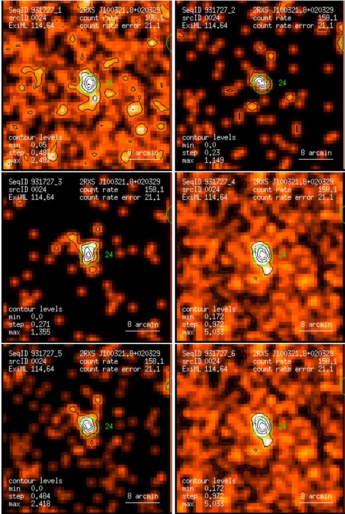
Figure 24: RASS 931727: detection 0024: band rate images, Gaussian filter: (1) PSPC channels 11 – 41, (2) 52 – 90, (3) 91 – 201, (4) 11 – 235, (5) 52 – 201, (6) 11 – 201. Broad band rates in counts/ks. Band rate contour levels in counts/ks/arcmin 2 .
