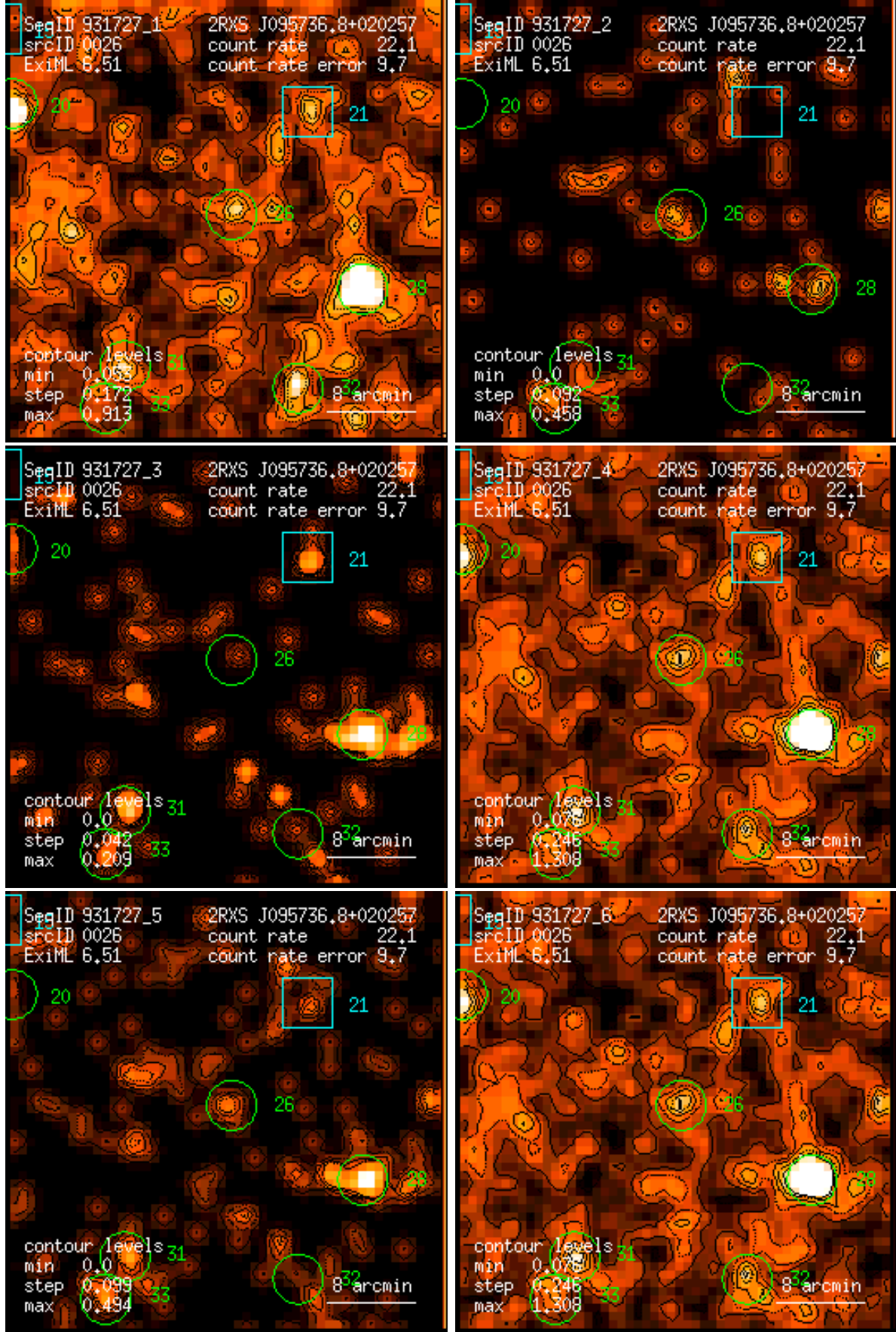
Figure 26: RASS 931727: detection 0026: band rate images, Gaussian filter: (1) PSPC channels 11 – 41, (2) 52 – 90, (3) 91 – 201, (4) 11 – 235, (5) 52 – 201, (6) 11 – 201. Broad band rates in counts/ks. Band rate contour levels in counts/ks/arcmin 2 .
