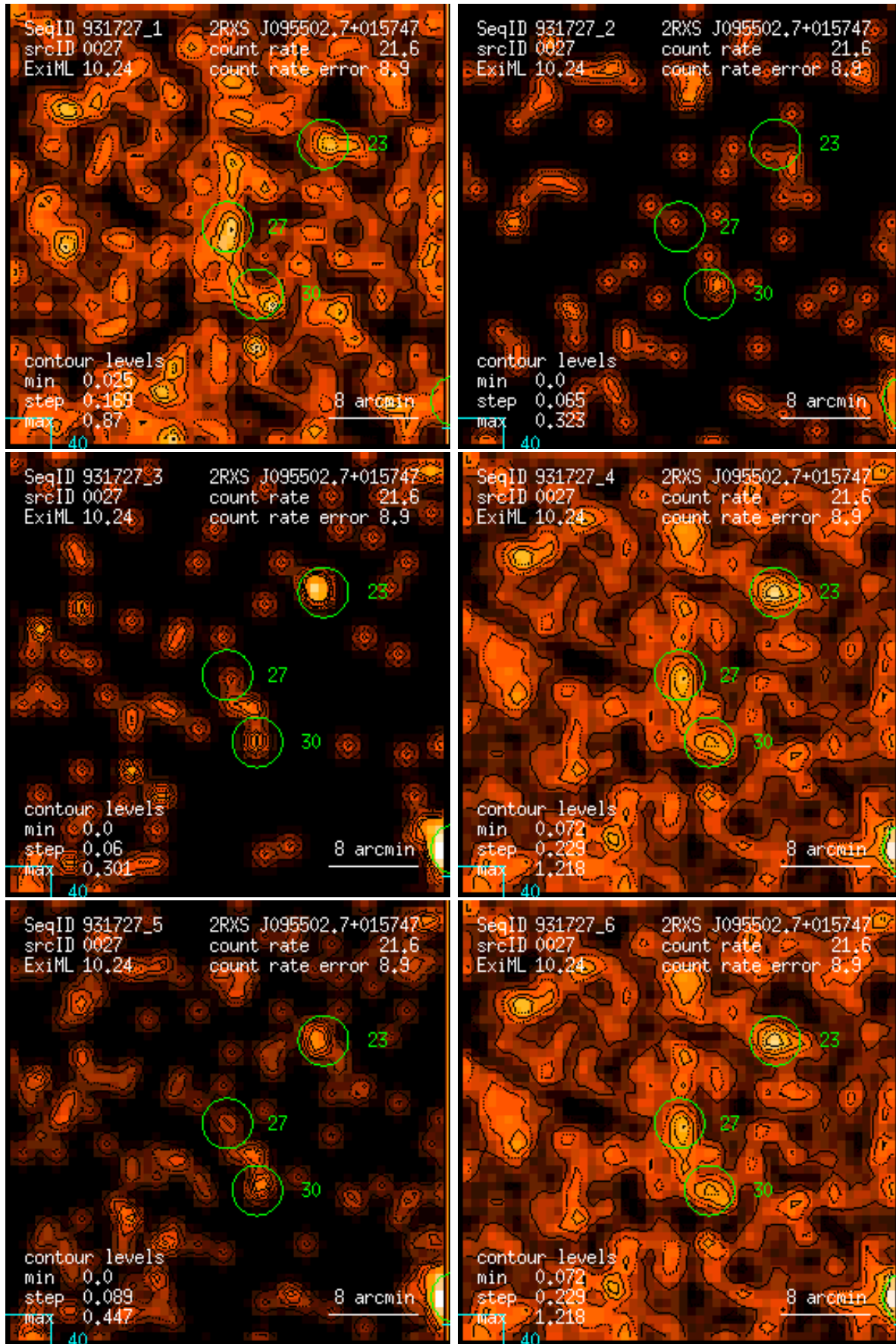
Figure 27: RASS 931727: detection 0027: band rate images, Gaussian filter: (1) PSPC channels 11 – 41, (2) 52 – 90, (3) 91 – 201, (4) 11 – 235, (5) 52 – 201, (6) 11 – 201. Broad band rates in counts/ks. Band rate contour levels in counts/ks/arcmin 2 .
