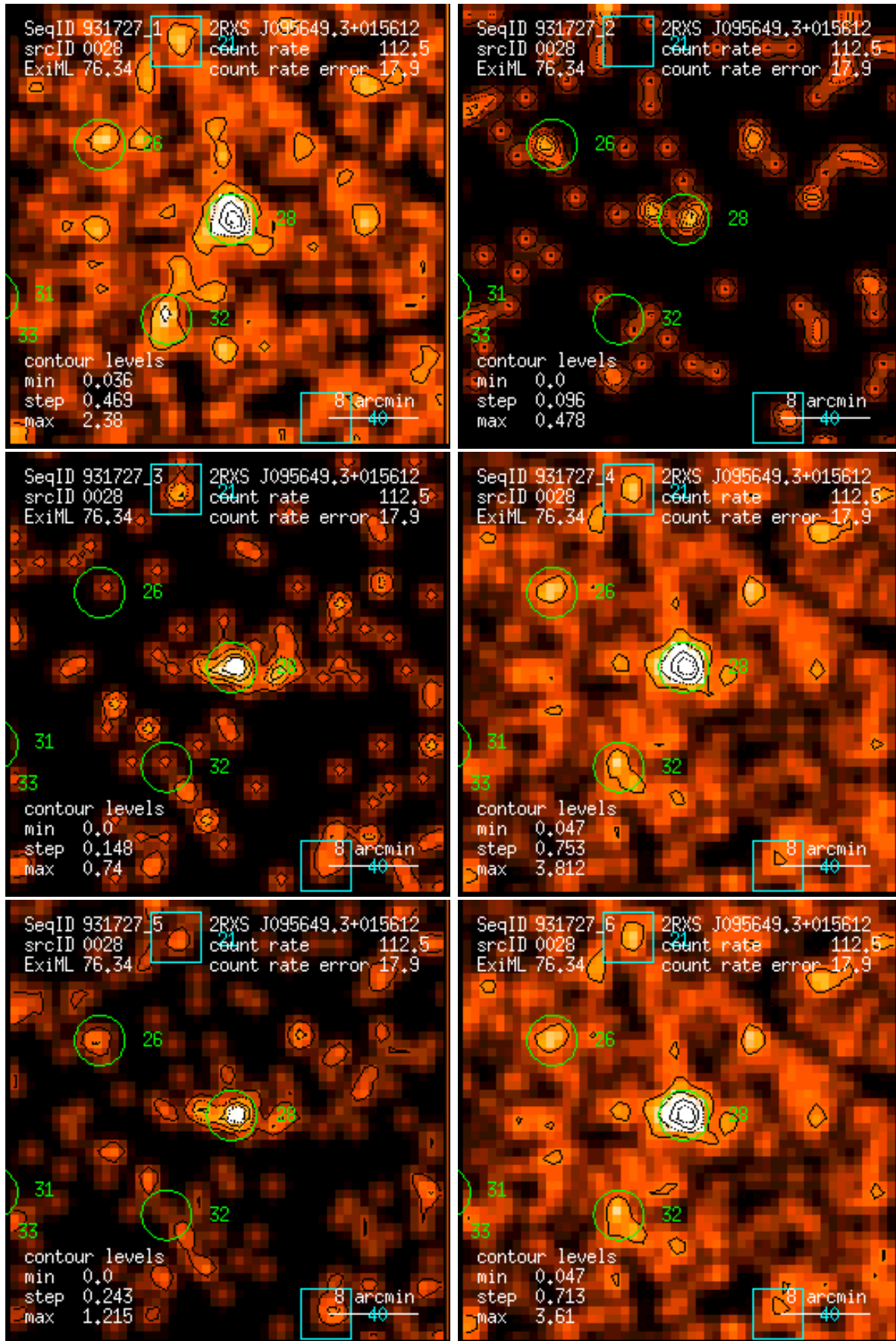
Figure 28: RASS 931727: detection 0028: band rate images, Gaussian filter: (1) PSPC channels 11 – 41, (2) 52 – 90, (3) 91 – 201, (4) 11 – 235, (5) 52 – 201, (6) 11 – 201. Broad band rates in counts/ks. Band rate contour levels in counts/ks/arcmin 2 .
