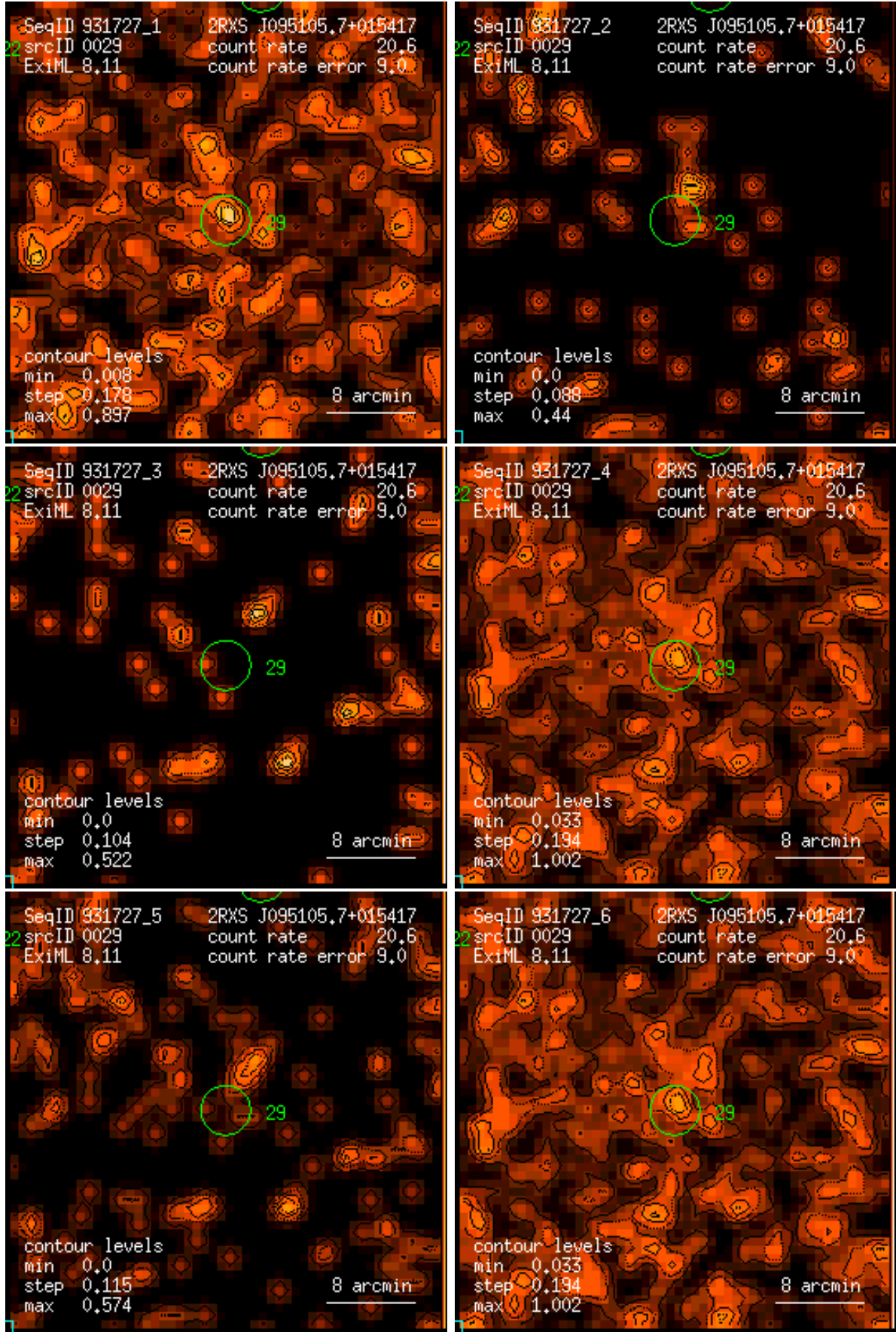
Figure 29: RASS 931727: detection 0029: band rate images, Gaussian filter: (1) PSPC channels 11 – 41, (2) 52 – 90, (3) 91 – 201, (4) 11 – 235, (5) 52 – 201, (6) 11 – 201. Broad band rates in counts/ks. Band rate contour levels in counts/ks/arcmin 2 .
