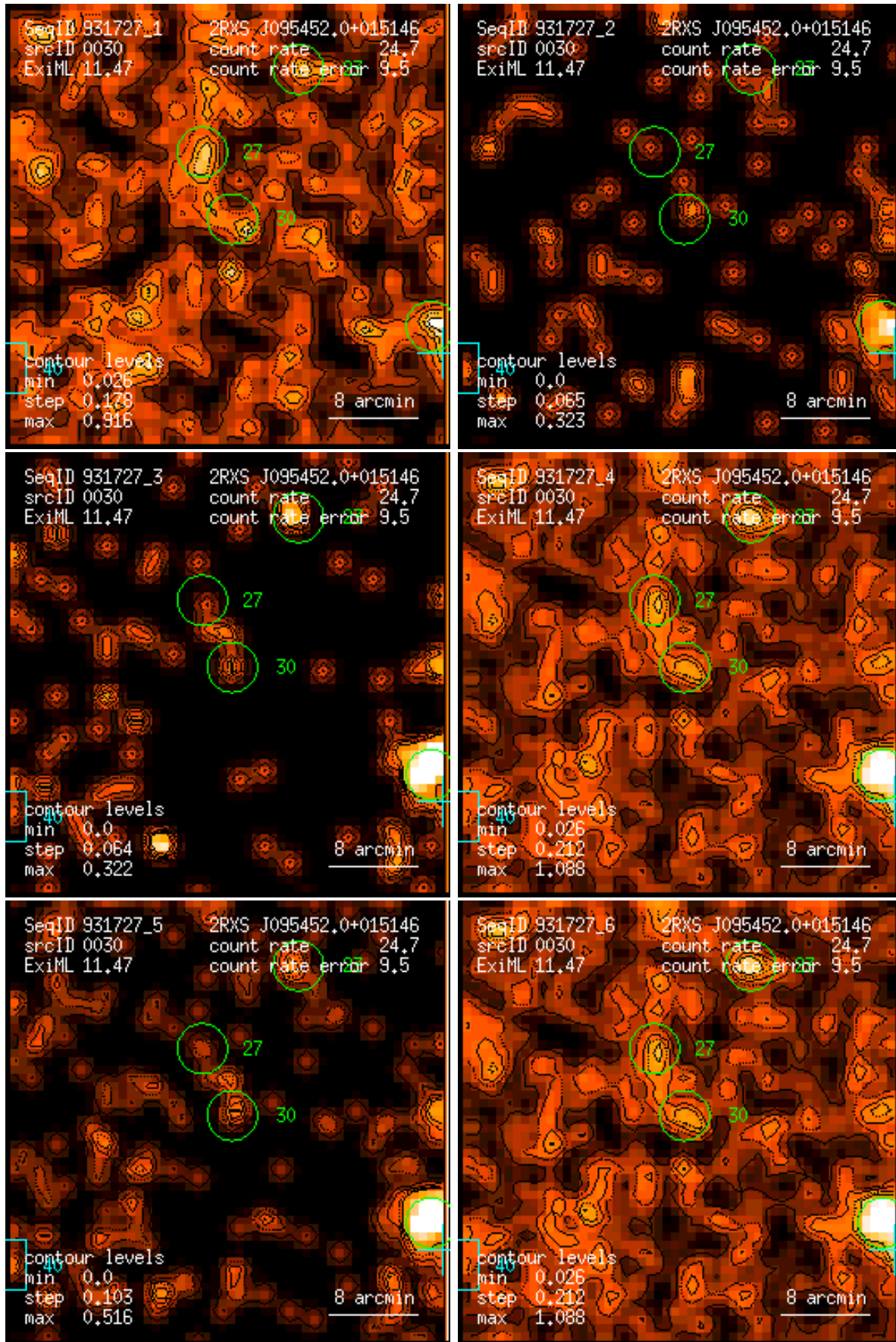
Figure 30: RASS 931727: detection 0030: band rate images, Gaussian filter: (1) PSPC channels 11 – 41, (2) 52 – 90, (3) 91 – 201, (4) 11 – 235, (5) 52 – 201, (6) 11 – 201. Broad band rates in counts/ks. Band rate contour levels in counts/ks/arcmin 2 .
