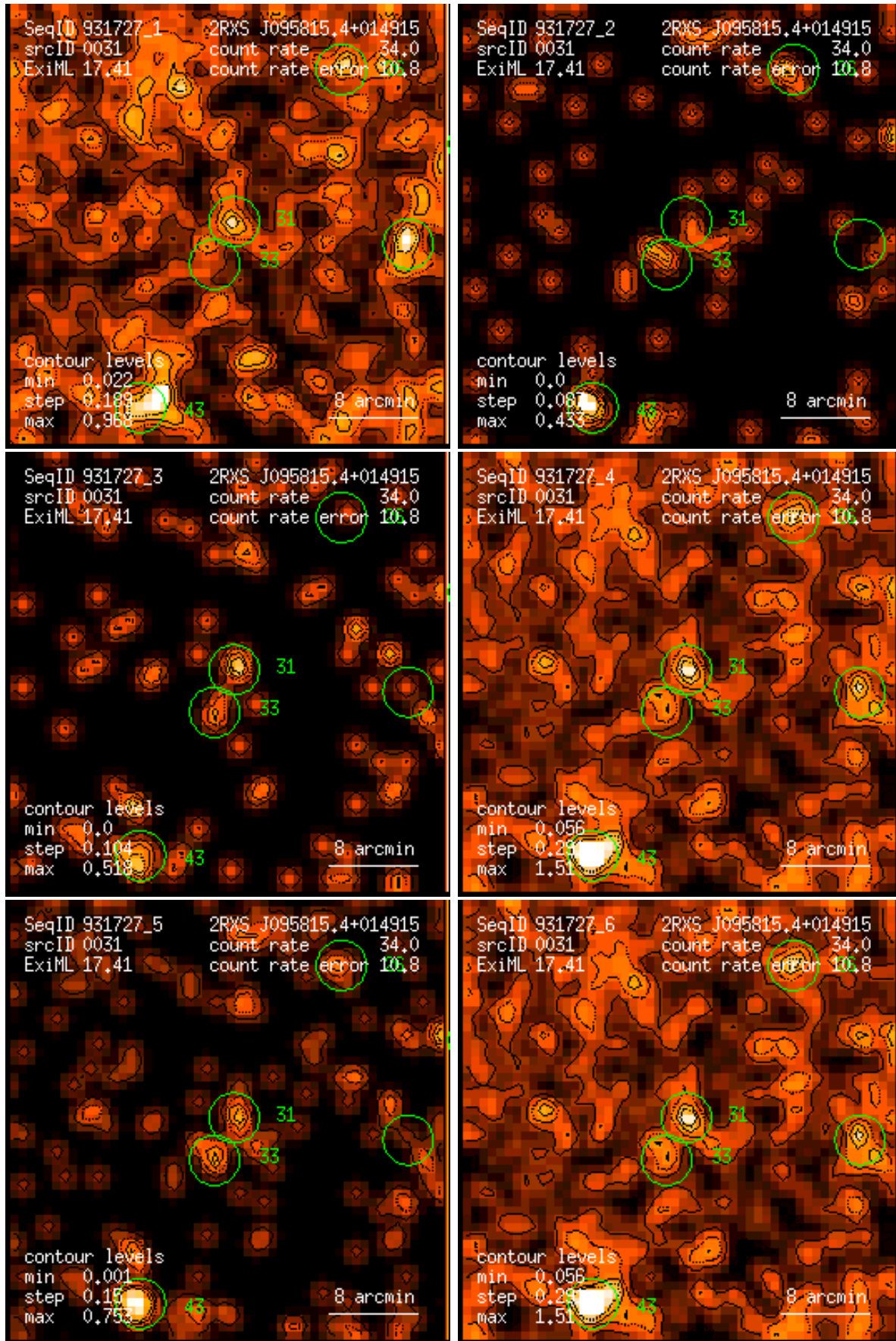
Figure 31: RASS 931727: detection 0031: band rate images, Gaussian filter: (1) PSPC channels 11 – 41, (2) 52 – 90, (3) 91 – 201, (4) 11 – 235, (5) 52 – 201, (6) 11 – 201. Broad band rates in counts/ks. Band rate contour levels in counts/ks/arcmin 2 .
