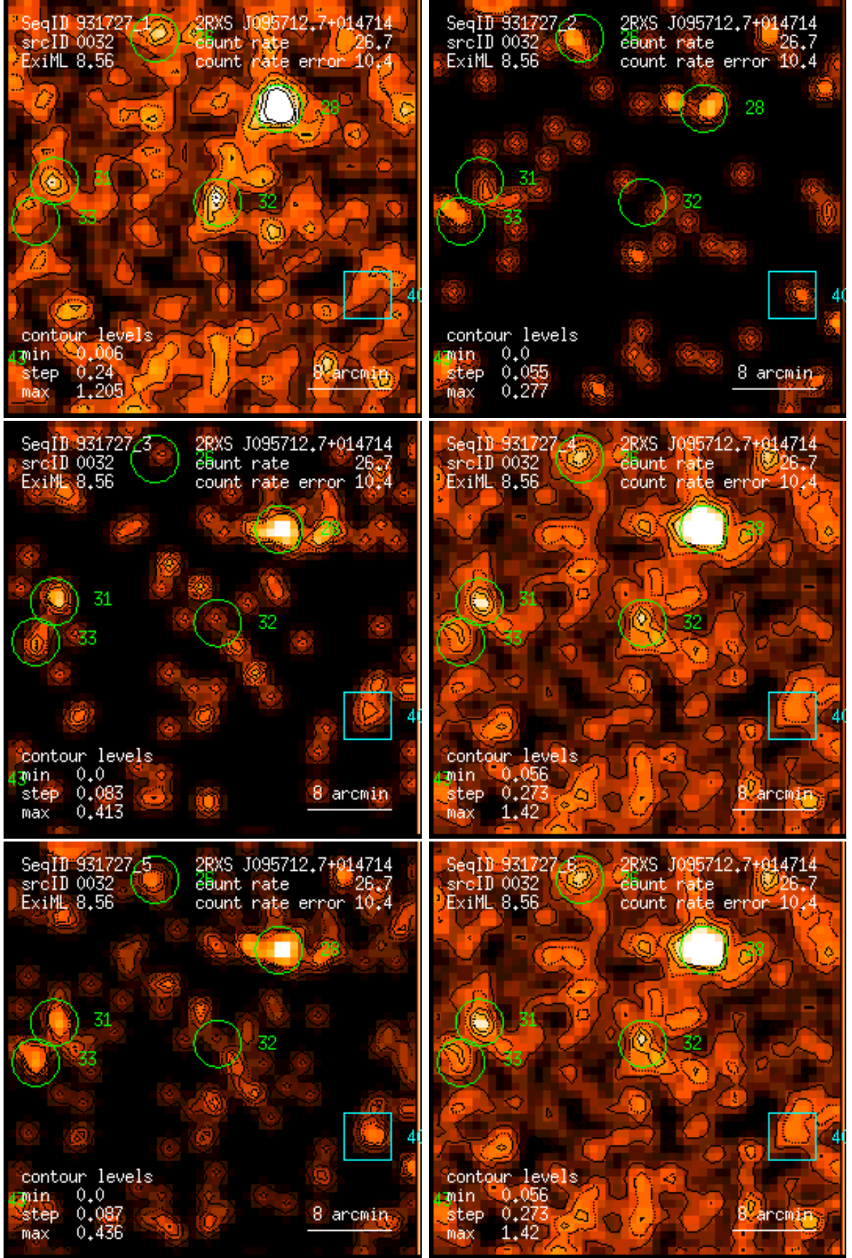
Figure 32: RASS 931727: detection 0032: band rate images, Gaussian filter: (1) PSPC channels 11 – 41, (2) 52 – 90, (3) 91 – 201, (4) 11 – 235, (5) 52 – 201, (6) 11 – 201. Broad band rates in counts/ks. Band rate contour levels in counts/ks/arcmin 2 .
