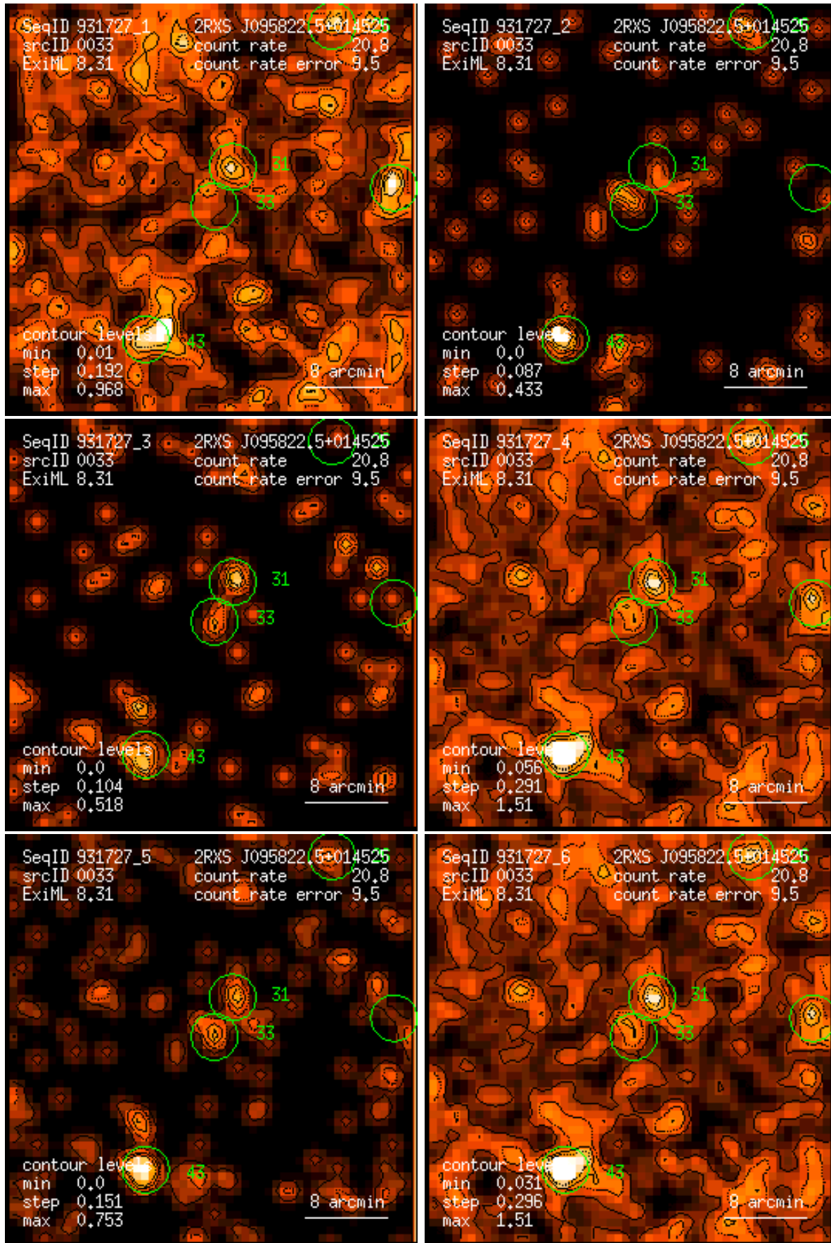
Figure 33: RASS 931727: detection 0033: band rate images, Gaussian filter: (1) PSPC channels 11 – 41, (2) 52 – 90, (3) 91 – 201, (4) 11 – 235, (5) 52 – 201, (6) 11 – 201. Broad band rates in counts/ks. Band rate contour levels in counts/ks/arcmin 2 .
