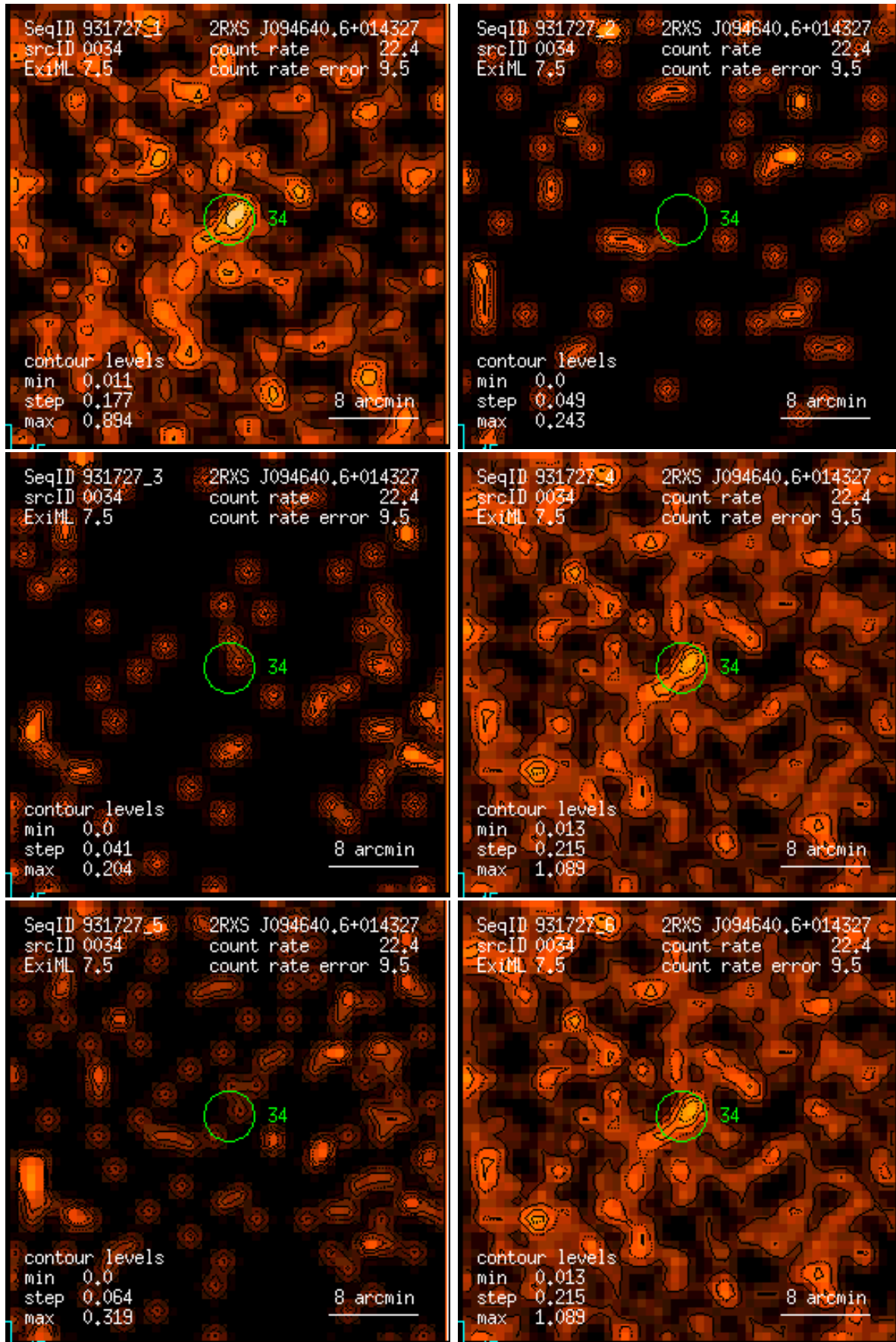
Figure 34: RASS 931727: detection 0034: band rate images, Gaussian filter: (1) PSPC channels 11 – 41, (2) 52 – 90, (3) 91 – 201, (4) 11 – 235, (5) 52 – 201, (6) 11 – 201. Broad band rates in counts/ks. Band rate contour levels in counts/ks/arcmin 2 .
