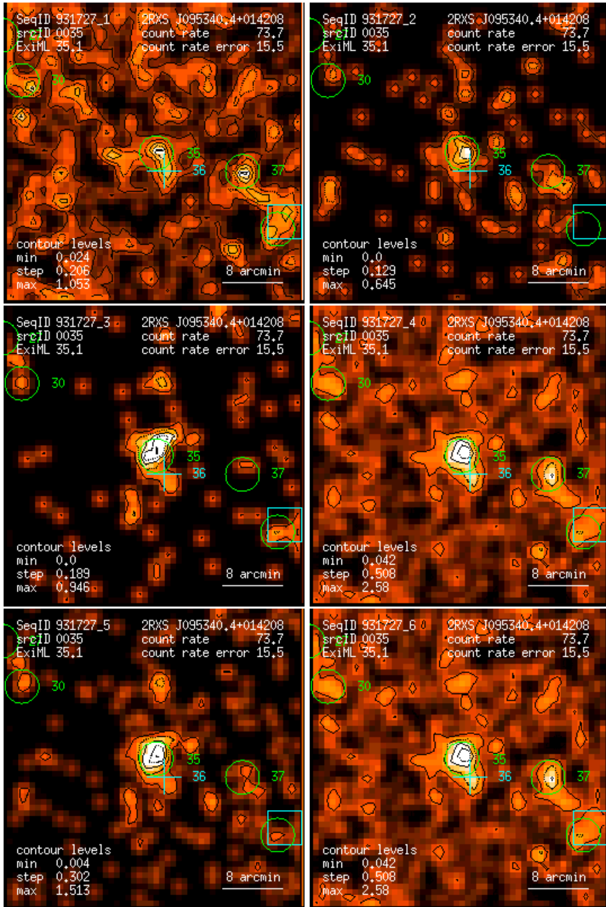
Figure 35: RASS 931727: detection 0035: band rate images, Gaussian filter: (1) PSPC channels 11 – 41, (2) 52 – 90, (3) 91 – 201, (4) 11 – 235, (5) 52 – 201, (6) 11 – 201. Broad band rates in counts/ks. Band rate contour levels in counts/ks/arcmin 2 .
