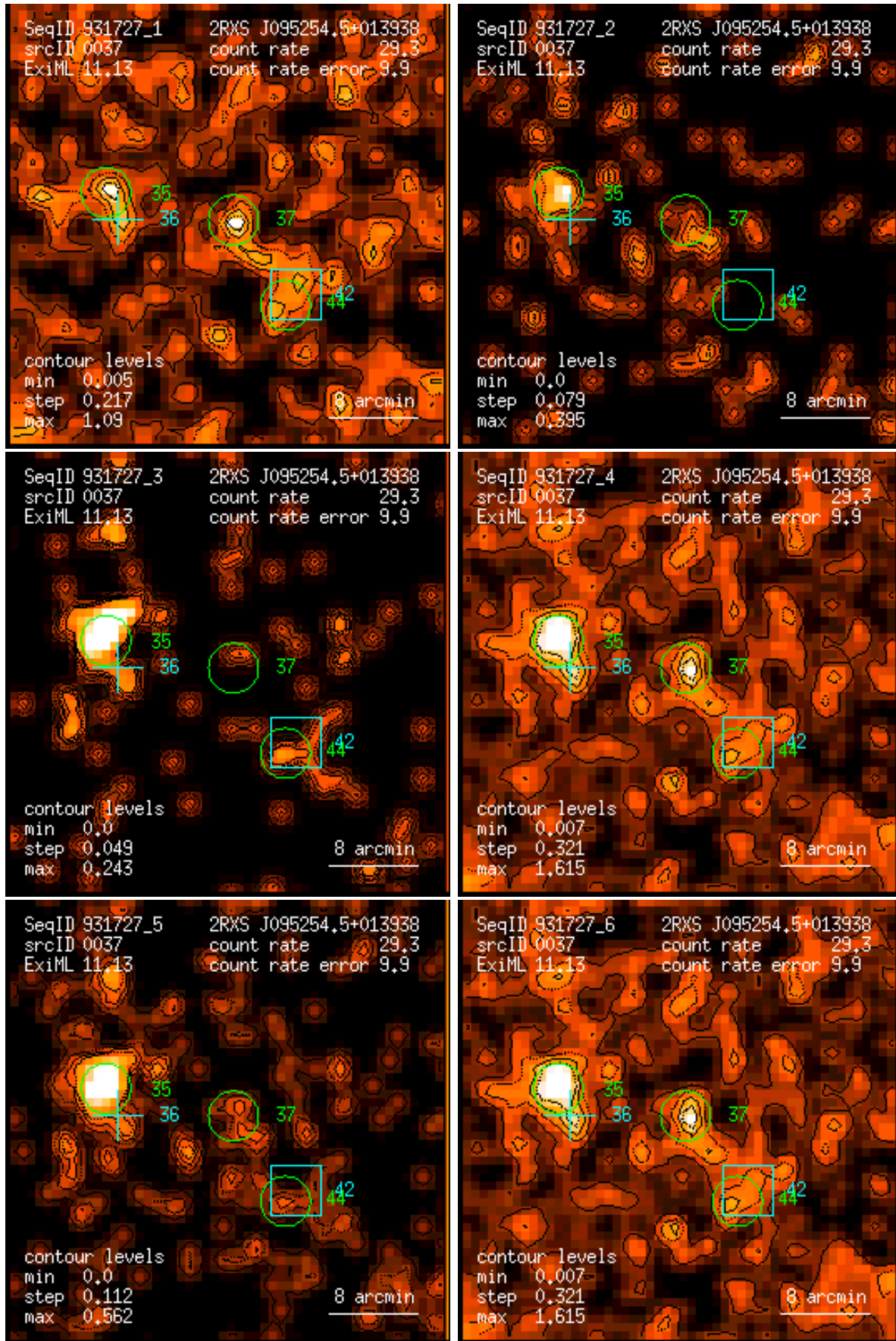
Figure 37: RASS 931727: detection 0037: band rate images, Gaussian filter: (1) PSPC channels 11 – 41, (2) 52 – 90, (3) 91 – 201, (4) 11 – 235, (5) 52 – 201, (6) 11 – 201. Broad band rates in counts/ks. Band rate contour levels in counts/ks/arcmin 2 .
