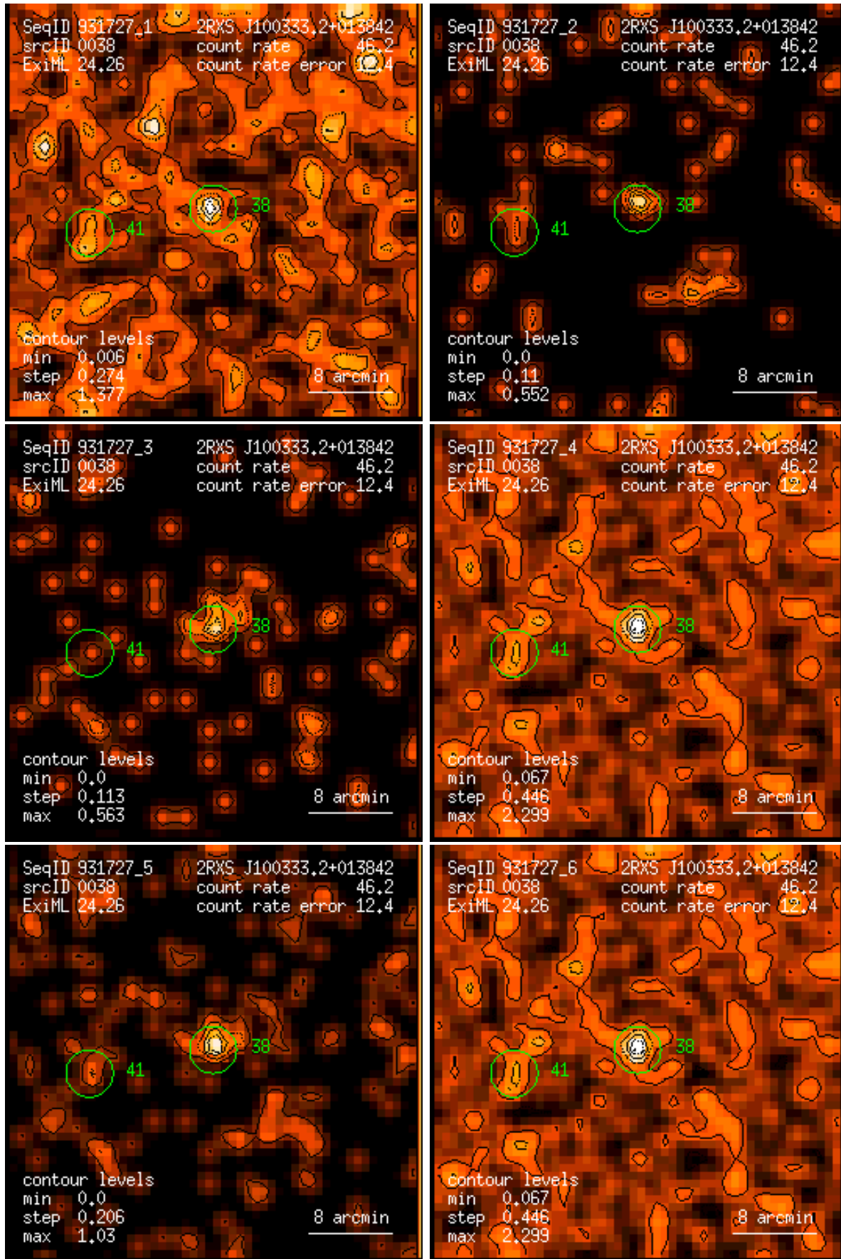
Figure 38: RASS 931727: detection 0038: band rate images, Gaussian filter: (1) PSPC channels 11 – 41, (2) 52 – 90, (3) 91 – 201, (4) 11 – 235, (5) 52 – 201, (6) 11 – 201. Broad band rates in counts/ks. Band rate contour levels in counts/ks/arcmin 2 .
