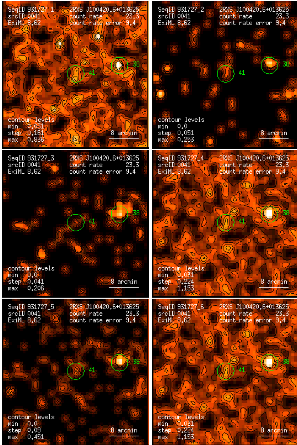
Figure 41: RASS 931727: detection 0041: band rate images, Gaussian filter: (1) PSPC channels 11 – 41, (2) 52 – 90, (3) 91 – 201, (4) 11 – 235, (5) 52 – 201, (6) 11 – 201. Broad band rates in counts/ks. Band rate contour levels in counts/ks/arcmin 2 .
