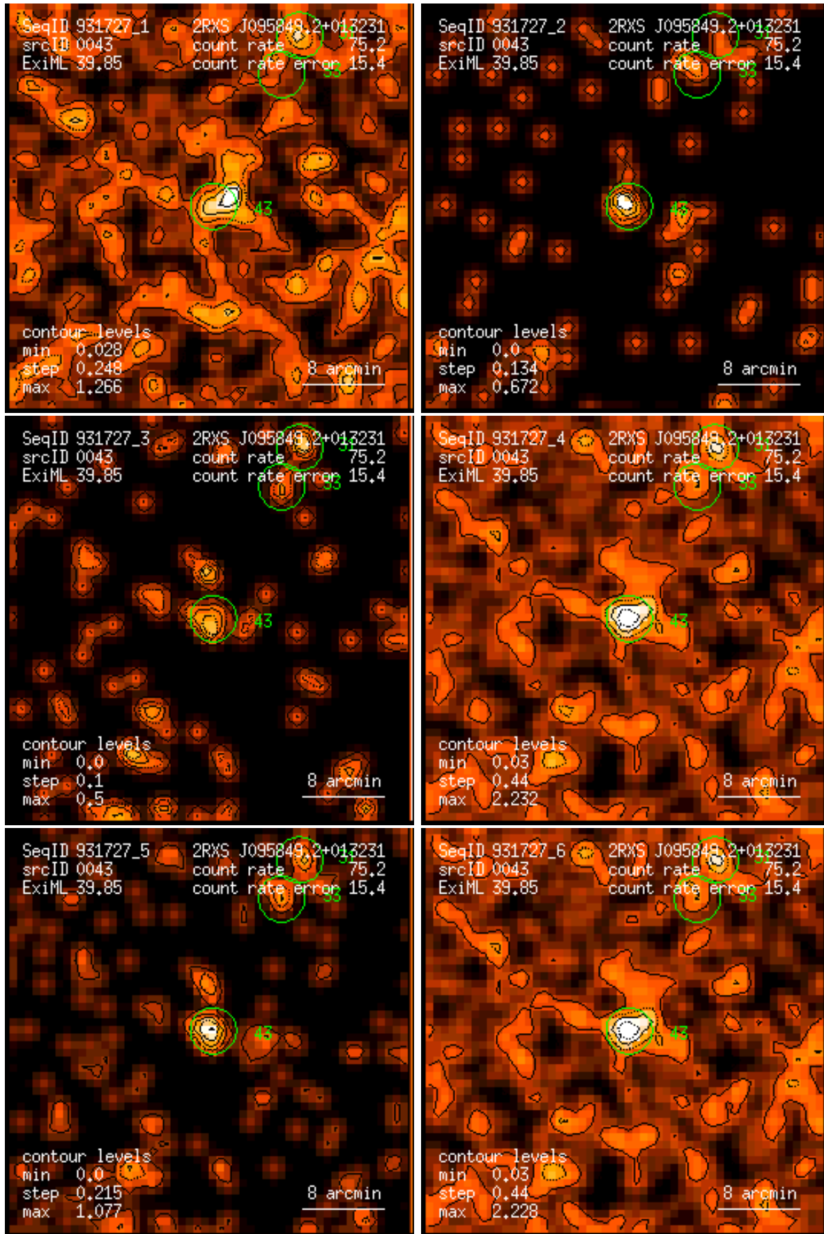
Figure 43: RASS 931727: detection 0043: band rate images, Gaussian filter: (1) PSPC channels 11 – 41, (2) 52 – 90, (3) 91 – 201, (4) 11 – 235, (5) 52 – 201, (6) 11 – 201. Broad band rates in counts/ks. Band rate contour levels in counts/ks/arcmin 2 .
