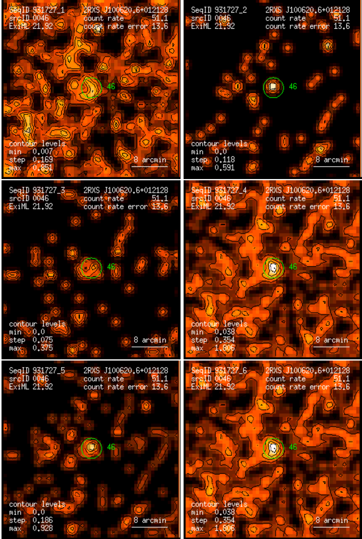
Figure 46: RASS 931727: detection 0046: band rate images, Gaussian filter: (1) PSPC channels 11 – 41, (2) 52 – 90, (3) 91 – 201, (4) 11 – 235, (5) 52 – 201, (6) 11 – 201. Broad band rates in counts/ks. Band rate contour levels in counts/ks/arcmin 2 .
