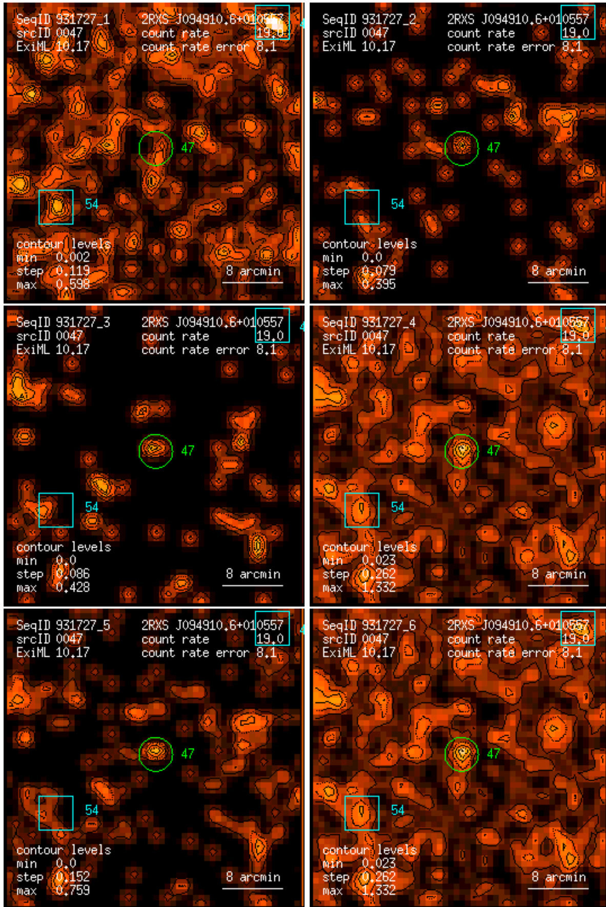
Figure 47: RASS 931727: detection 0047: band rate images, Gaussian filter: (1) PSPC channels 11 – 41, (2) 52 – 90, (3) 91 – 201, (4) 11 – 235, (5) 52 – 201, (6) 11 – 201. Broad band rates in counts/ks. Band rate contour levels in counts/ks/arcmin 2 .
