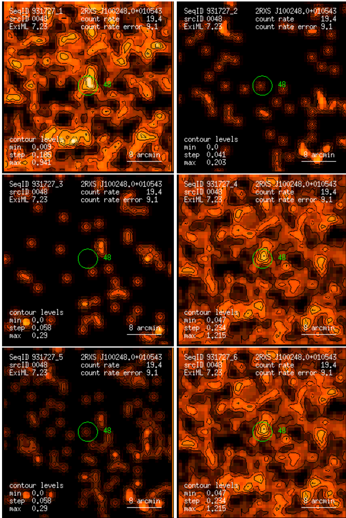
Figure 48: RASS 931727: detection 0048: band rate images, Gaussian filter: (1) PSPC channels 11 – 41, (2) 52 – 90, (3) 91 – 201, (4) 11 – 235, (5) 52 – 201, (6) 11 – 201. Broad band rates in counts/ks. Band rate contour levels in counts/ks/arcmin 2 .
