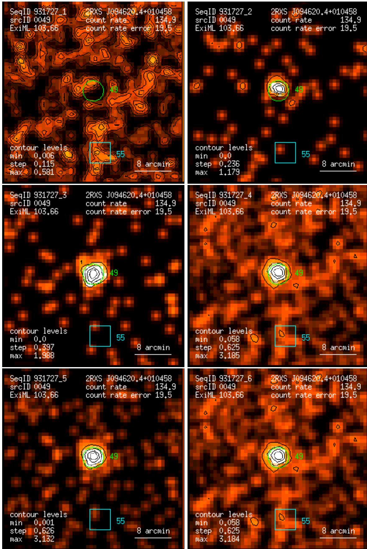
Figure 49: RASS 931727: detection 0049: band rate images, Gaussian filter: (1) PSPC channels 11 – 41, (2) 52 – 90, (3) 91 – 201, (4) 11 – 235, (5) 52 – 201, (6) 11 – 201. Broad band rates in counts/ks. Band rate contour levels in counts/ks/arcmin 2 .
