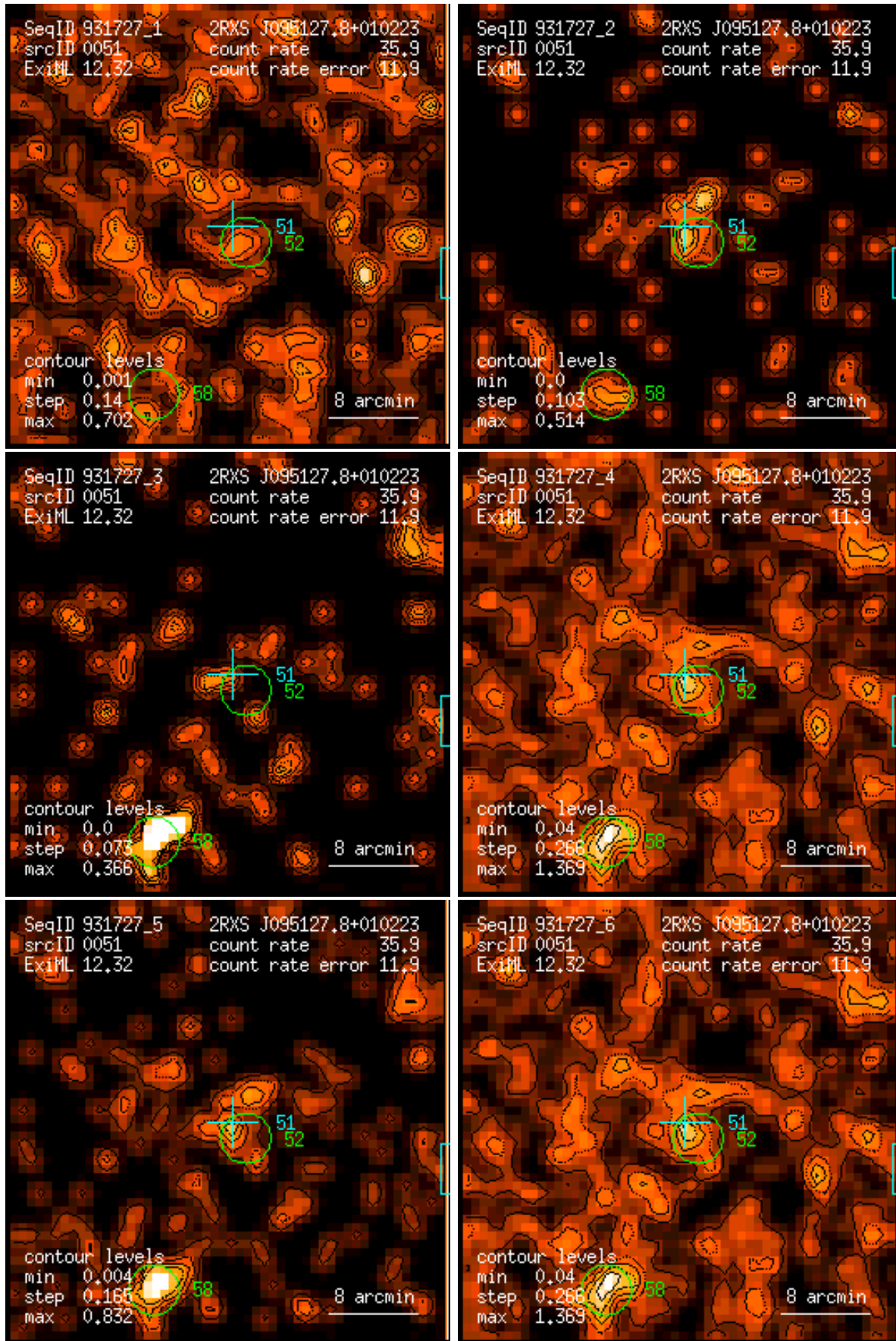
Figure 51: RASS 931727: detection 0051: band rate images, Gaussian filter: (1) PSPC channels 11 – 41, (2) 52 – 90, (3) 91 – 201, (4) 11 – 235, (5) 52 – 201, (6) 11 – 201. Broad band rates in counts/ks. Band rate contour levels in counts/ks/arcmin 2 .
