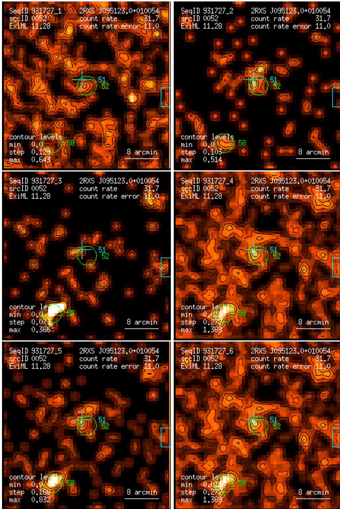
Figure 52: RASS 931727: detection 0052: band rate images, Gaussian filter: (1) PSPC channels 11 – 41, (2) 52 – 90, (3) 91 – 201, (4) 11 – 235, (5) 52 – 201, (6) 11 – 201. Broad band rates in counts/ks. Band rate contour levels in counts/ks/arcmin 2 .
