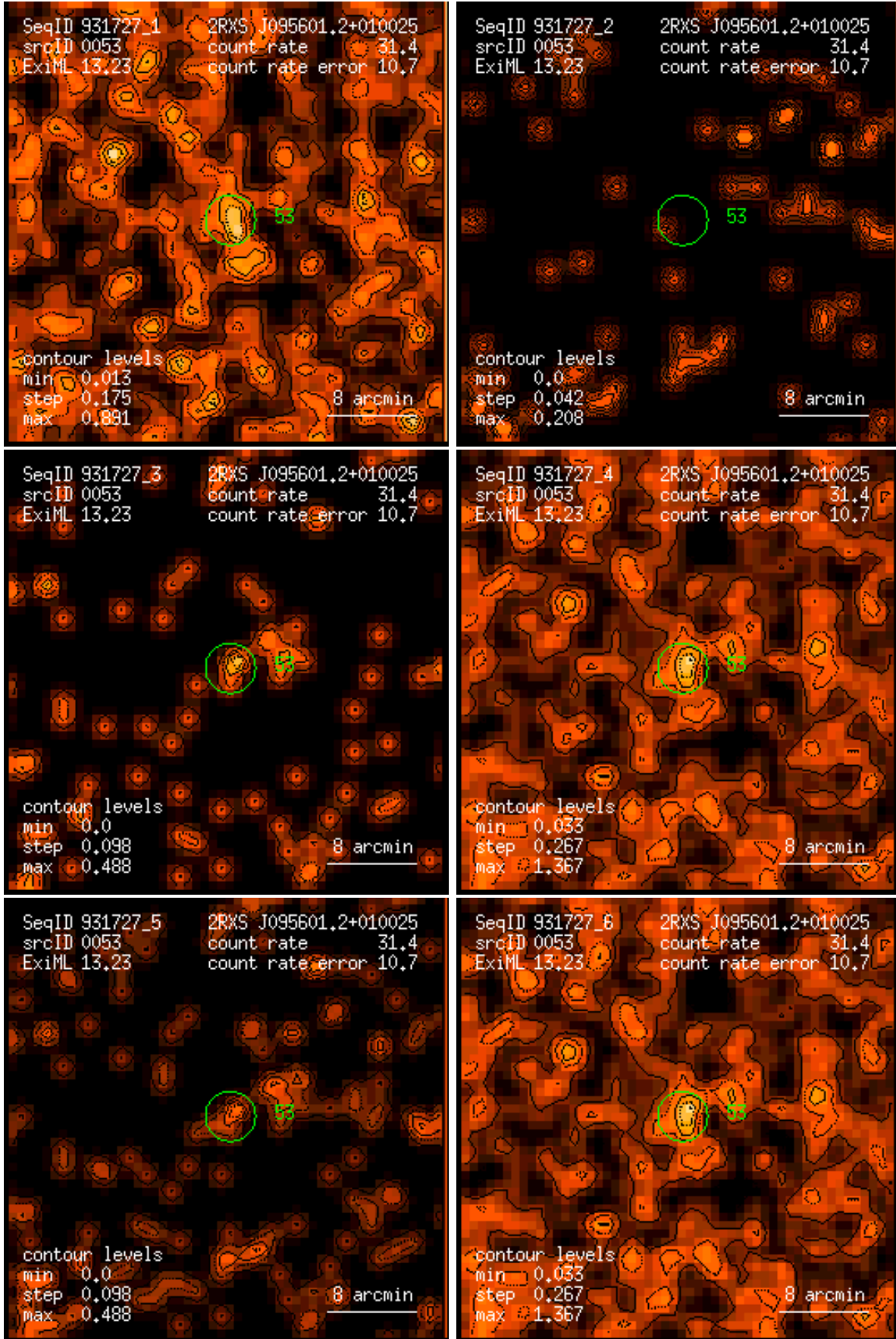
Figure 53: RASS 931727: detection 0053: band rate images, Gaussian filter: (1) PSPC channels 11 – 41, (2) 52 – 90, (3) 91 – 201, (4) 11 – 235, (5) 52 – 201, (6) 11 – 201. Broad band rates in counts/ks. Band rate contour levels in counts/ks/arcmin 2 .
