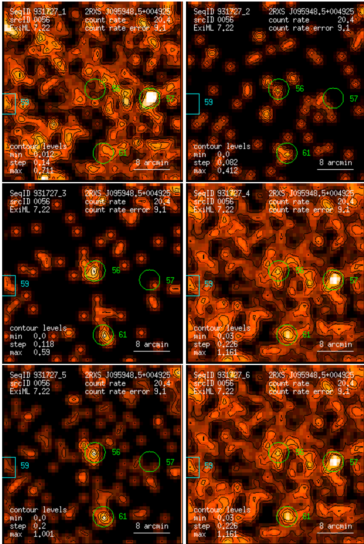
Figure 56: RASS 931727: detection 0056: band rate images, Gaussian filter: (1) PSPC channels 11 – 41, (2) 52 – 90, (3) 91 – 201, (4) 11 – 235, (5) 52 – 201, (6) 11 – 201. Broad band rates in counts/ks. Band rate contour levels in counts/ks/arcmin 2 .
