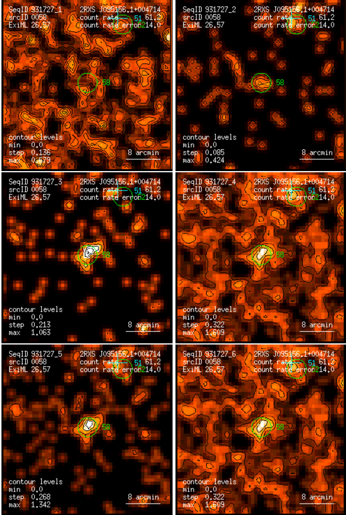
Figure 58: RASS 931727: detection 0058: band rate images, Gaussian filter: (1) PSPC channels 11 – 41, (2) 52 – 90, (3) 91 – 201, (4) 11 – 235, (5) 52 – 201, (6) 11 – 201. Broad band rates in counts/ks. Band rate contour levels in counts/ks/arcmin 2 .
