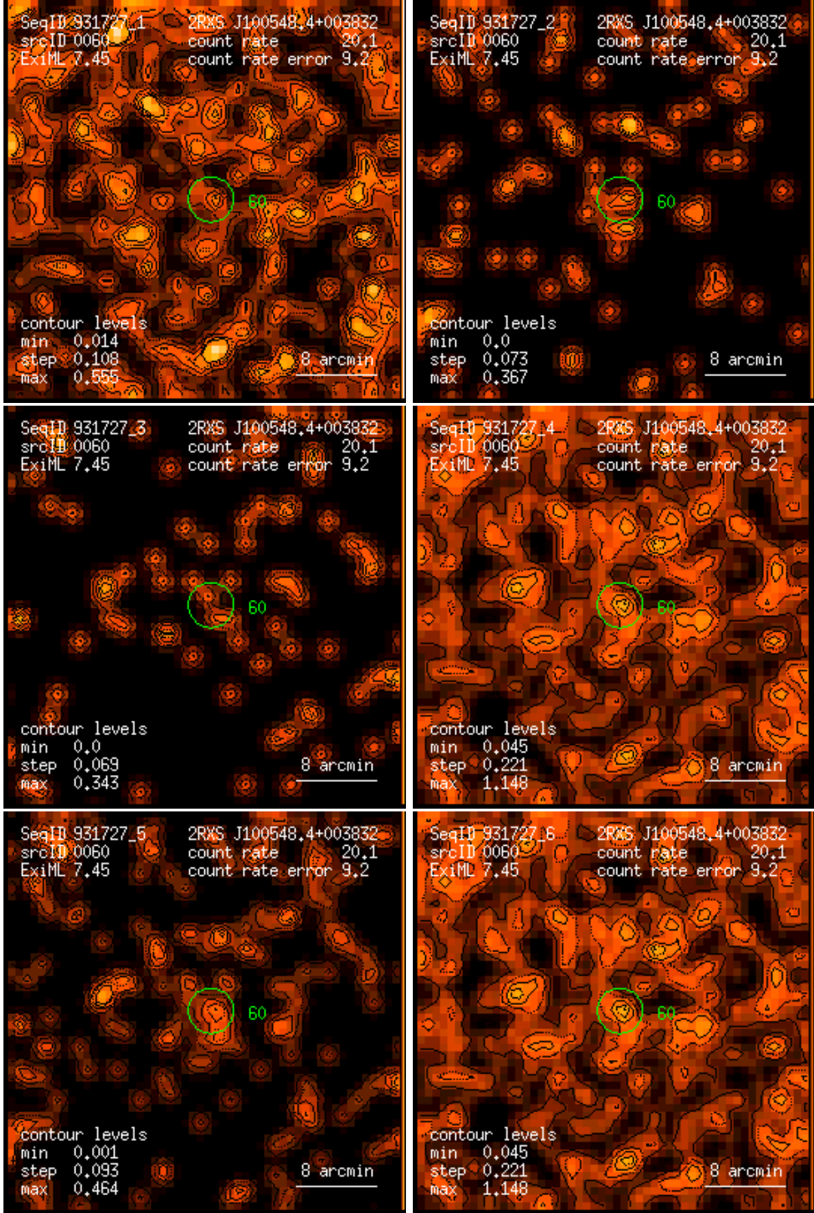
Figure 60: RASS 931727: detection 0060: band rate images, Gaussian filter: (1) PSPC channels 11 – 41, (2) 52 – 90, (3) 91 – 201, (4) 11 – 235, (5) 52 – 201, (6) 11 – 201. Broad band rates in counts/ks. Band rate contour levels in counts/ks/arcmin 2 .
