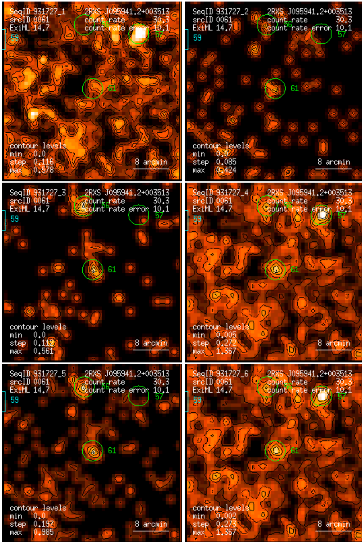
Figure 61: RASS 931727: detection 0061: band rate images, Gaussian filter: (1) PSPC channels 11 – 41, (2) 52 – 90, (3) 91 – 201, (4) 11 – 235, (5) 52 – 201, (6) 11 – 201. Broad band rates in counts/ks. Band rate contour levels in counts/ks/arcmin 2 .
