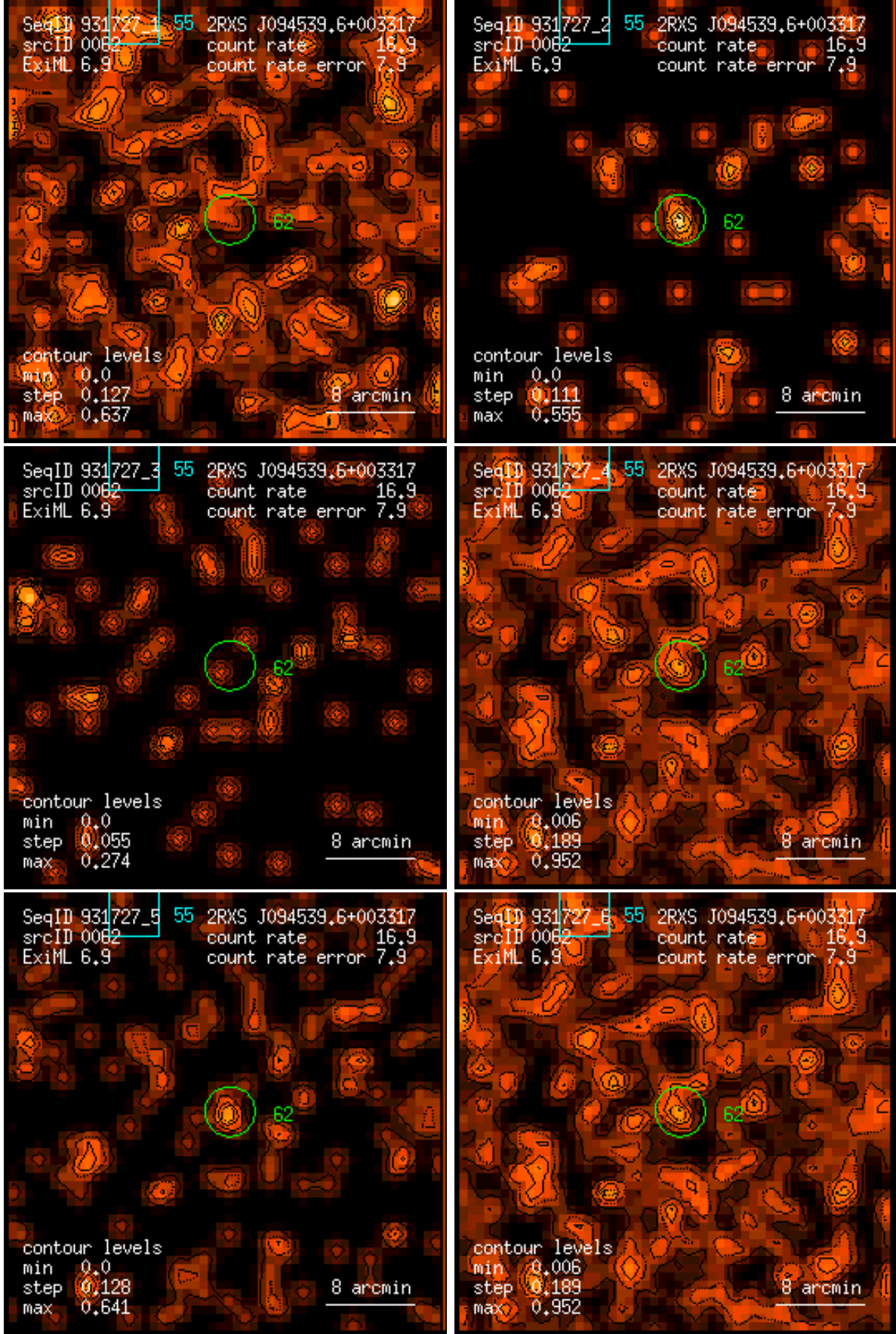
Figure 62: RASS 931727: detection 0062: band rate images, Gaussian filter: (1) PSPC channels 11 – 41, (2) 52 – 90, (3) 91 – 201, (4) 11 – 235, (5) 52 – 201, (6) 11 – 201. Broad band rates in counts/ks. Band rate contour levels in counts/ks/arcmin 2 .
