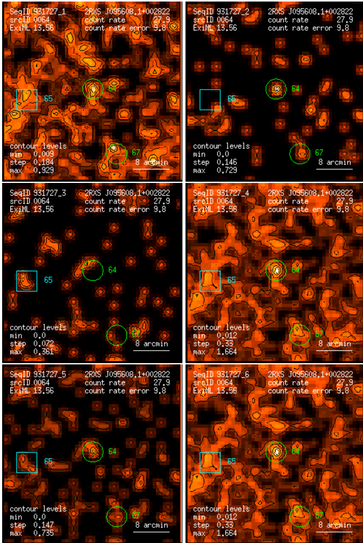
Figure 64: RASS 931727: detection 0064: band rate images, Gaussian filter: (1) PSPC channels 11 – 41, (2) 52 – 90, (3) 91 – 201, (4) 11 – 235, (5) 52 – 201, (6) 11 – 201. Broad band rates in counts/ks. Band rate contour levels in counts/ks/arcmin 2 .
