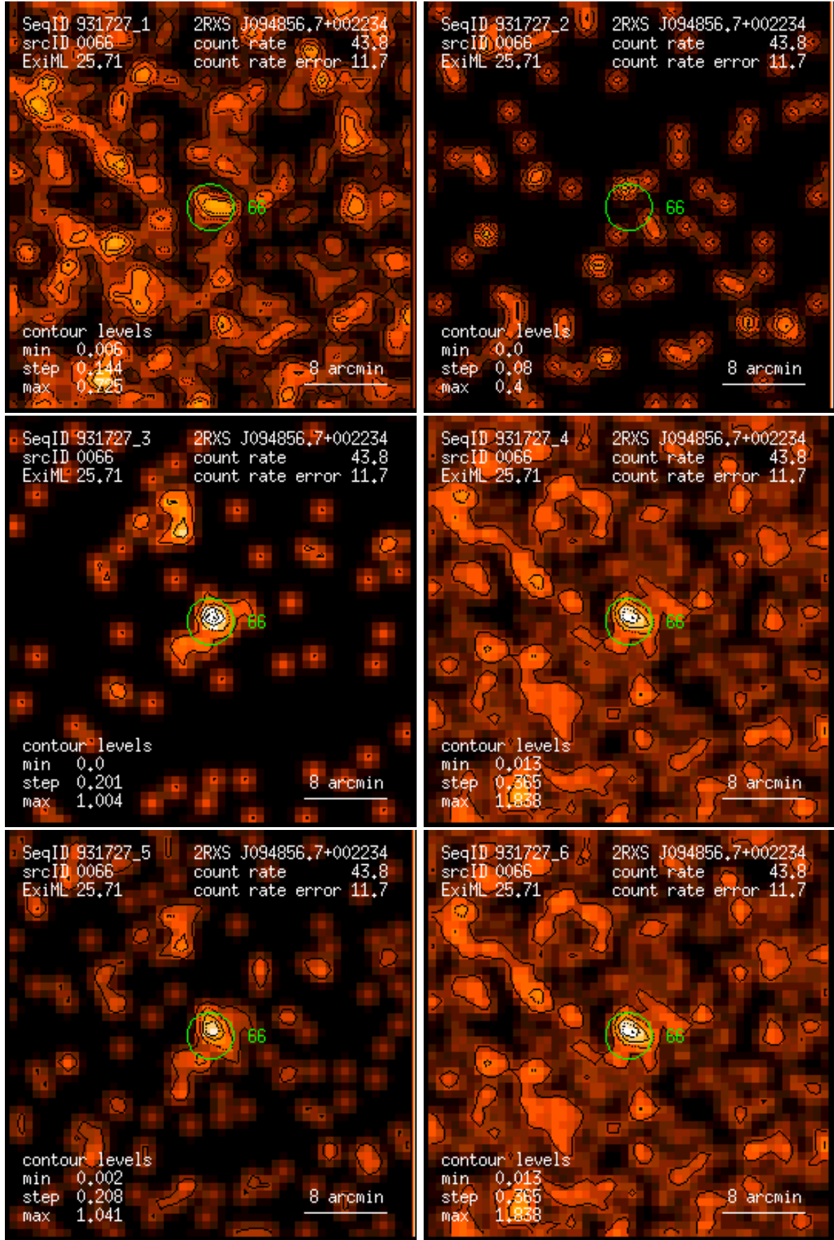
Figure 66: RASS 931727: detection 0066: band rate images, Gaussian filter: (1) PSPC channels 11 – 41, (2) 52 – 90, (3) 91 – 201, (4) 11 – 235, (5) 52 – 201, (6) 11 – 201. Broad band rates in counts/ks. Band rate contour levels in counts/ks/arcmin 2 .
