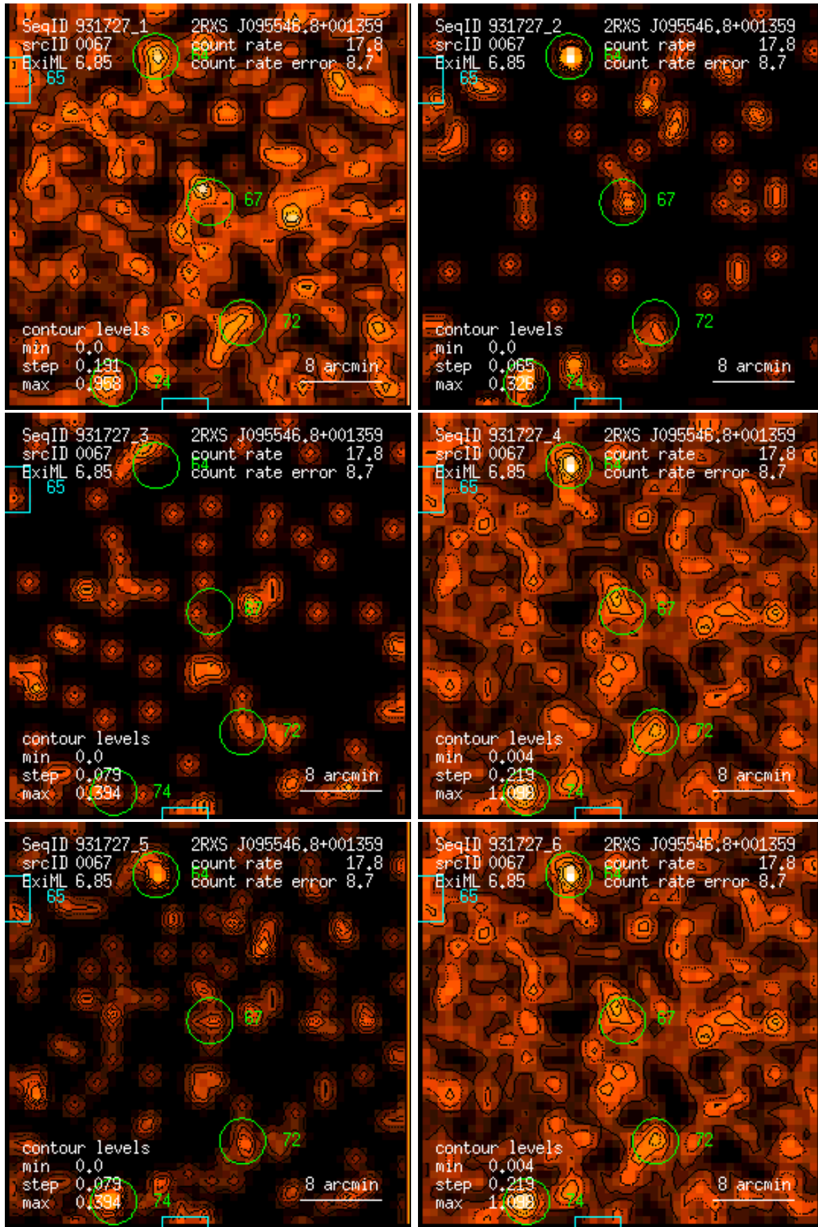
Figure 67: RASS 931727: detection 0067: band rate images, Gaussian filter: (1) PSPC channels 11 – 41, (2) 52 – 90, (3) 91 – 201, (4) 11 – 235, (5) 52 – 201, (6) 11 – 201. Broad band rates in counts/ks. Band rate contour levels in counts/ks/arcmin 2 .
