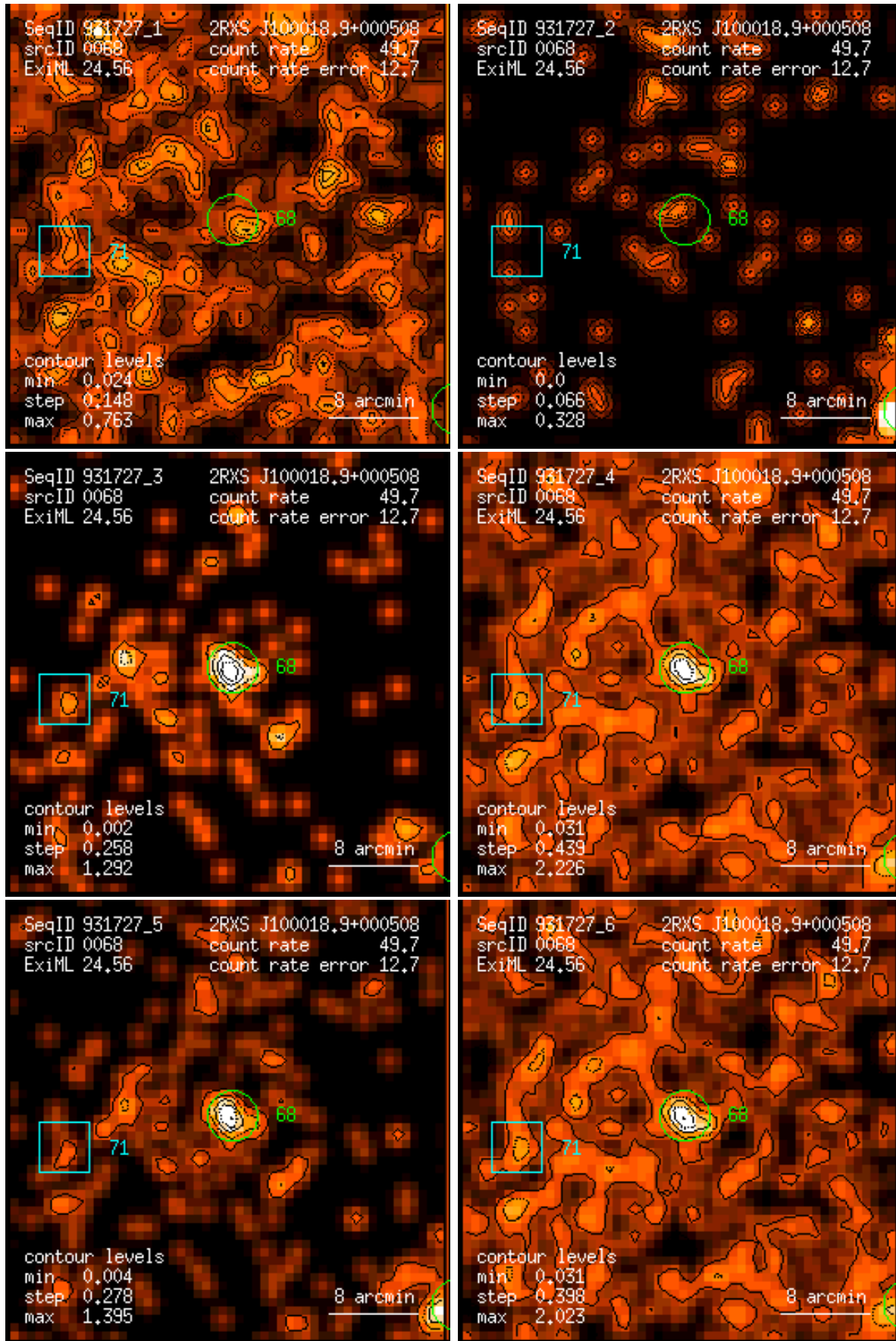
Figure 68: RASS 931727: detection 0068: band rate images, Gaussian filter: (1) PSPC channels 11 – 41, (2) 52 – 90, (3) 91 – 201, (4) 11 – 235, (5) 52 – 201, (6) 11 – 201. Broad band rates in counts/ks. Band rate contour levels in counts/ks/arcmin 2 .
