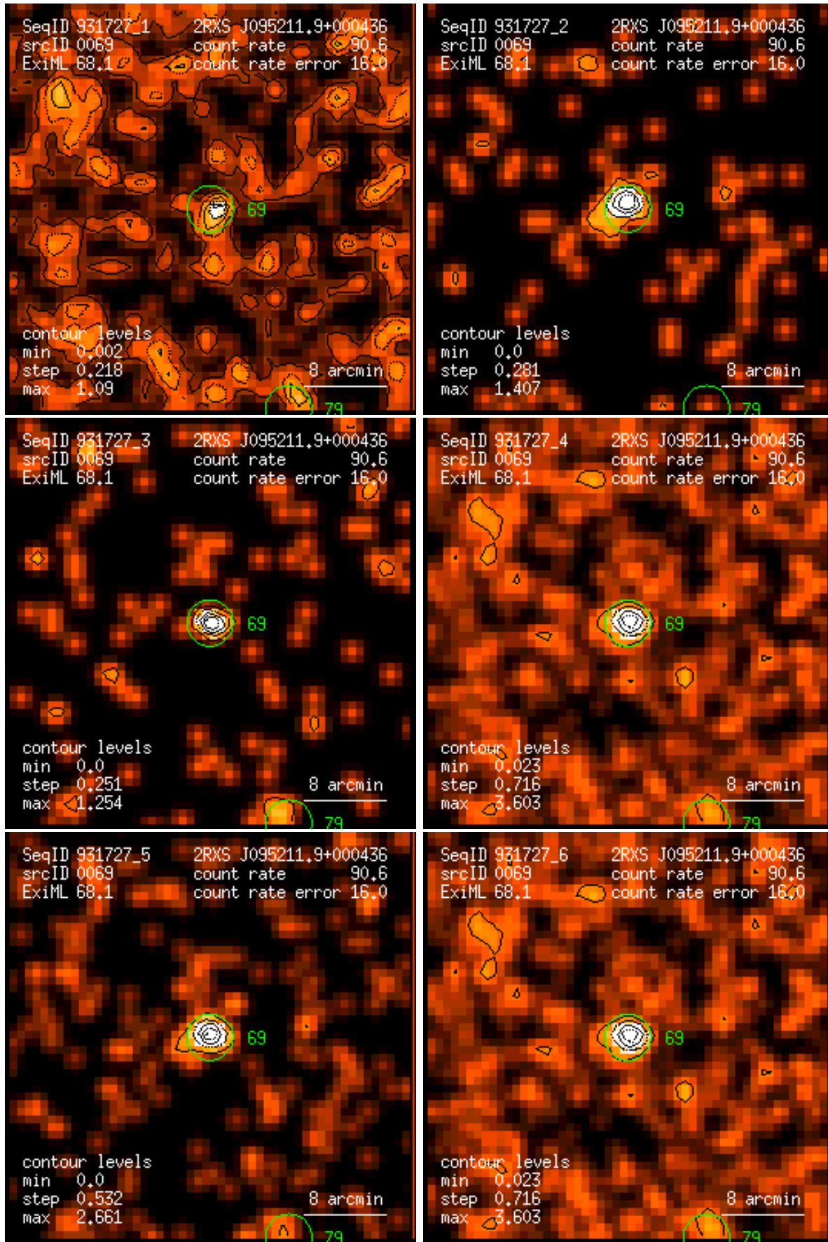
Figure 69: RASS 931727: detection 0069: band rate images, Gaussian filter: (1) PSPC channels 11 – 41, (2) 52 – 90, (3) 91 – 201, (4) 11 – 235, (5) 52 – 201, (6) 11 – 201. Broad band rates in counts/ks. Band rate contour levels in counts/ks/arcmin 2 .
