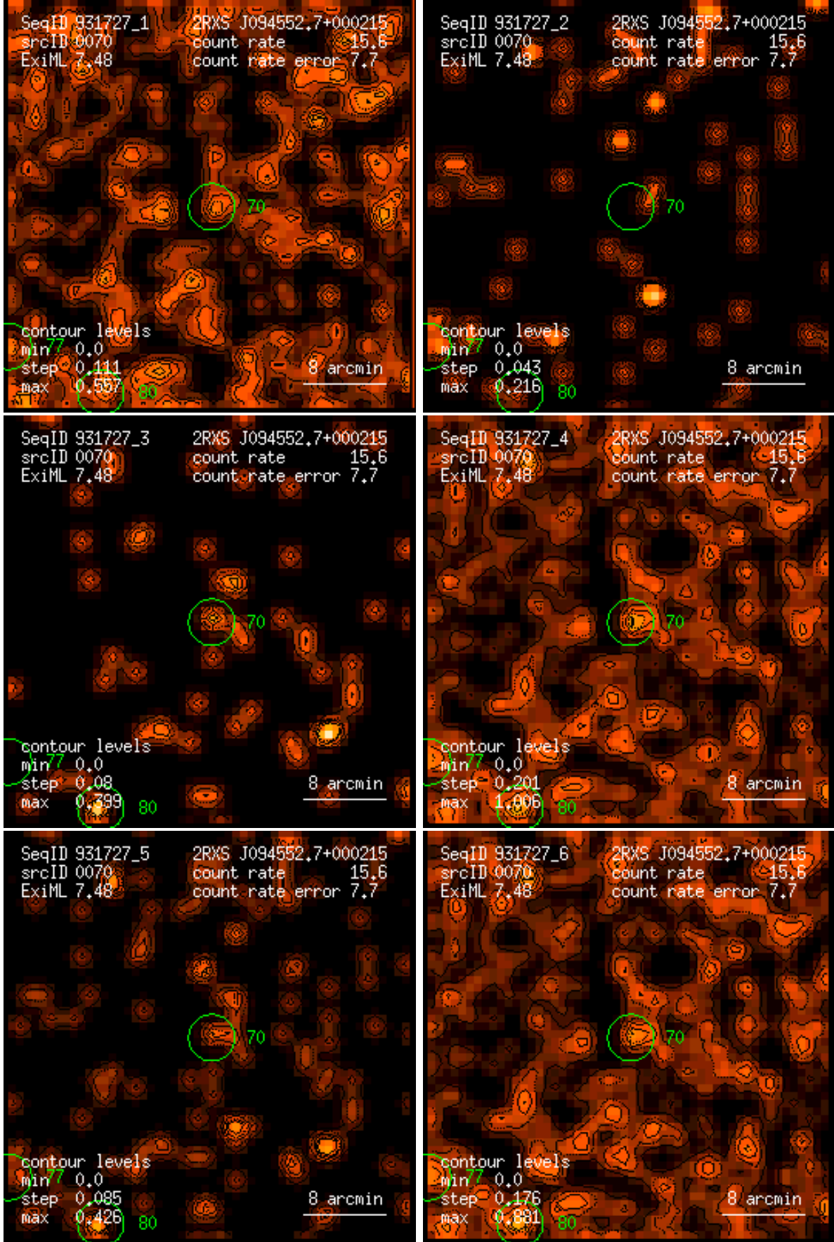
Figure 70: RASS 931727: detection 0070: band rate images, Gaussian filter: (1) PSPC channels 11 – 41, (2) 52 – 90, (3) 91 – 201, (4) 11 – 235, (5) 52 – 201, (6) 11 – 201. Broad band rates in counts/ks. Band rate contour levels in counts/ks/arcmin 2 .
