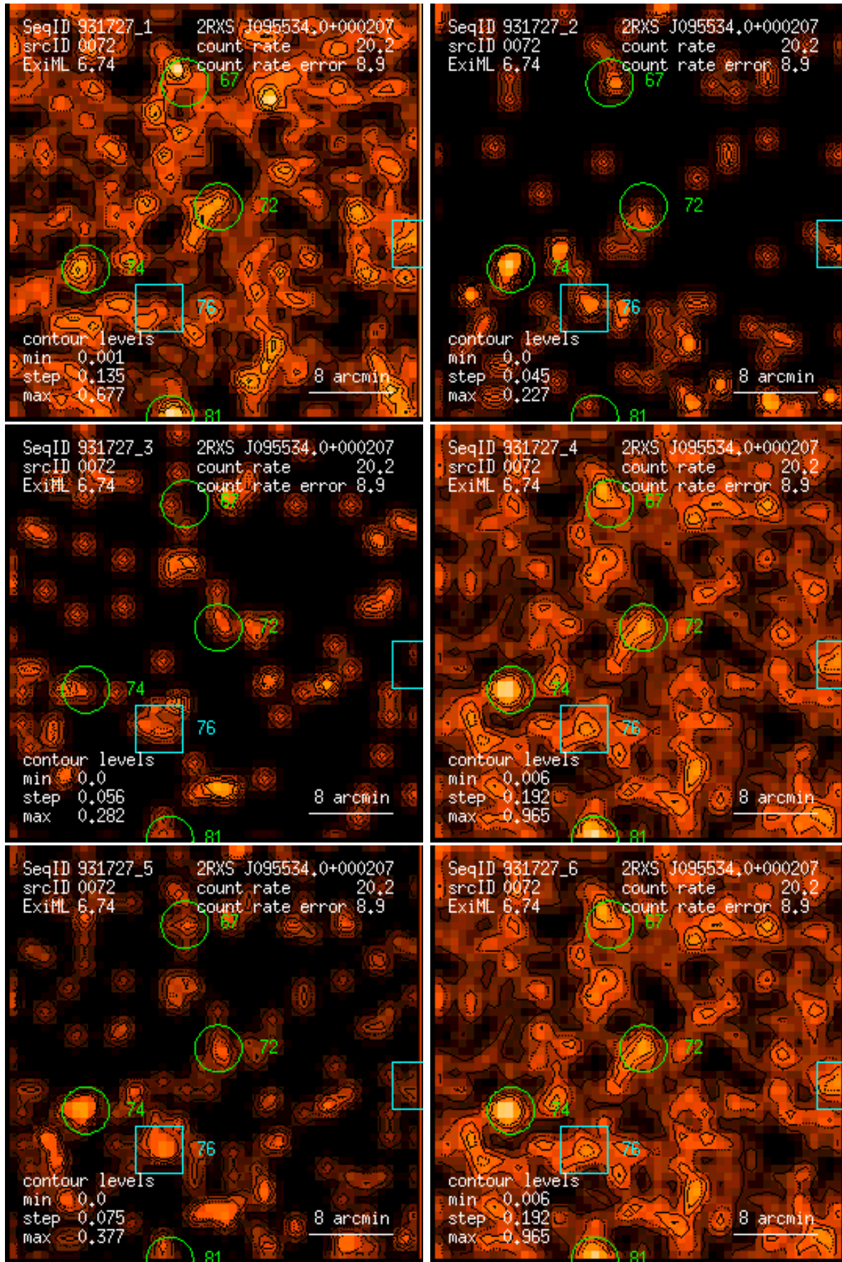
Figure 72: RASS 931727: detection 0072: band rate images, Gaussian filter: (1) PSPC channels 11 – 41, (2) 52 – 90, (3) 91 – 201, (4) 11 – 235, (5) 52 – 201, (6) 11 – 201. Broad band rates in counts/ks. Band rate contour levels in counts/ks/arcmin 2 .
