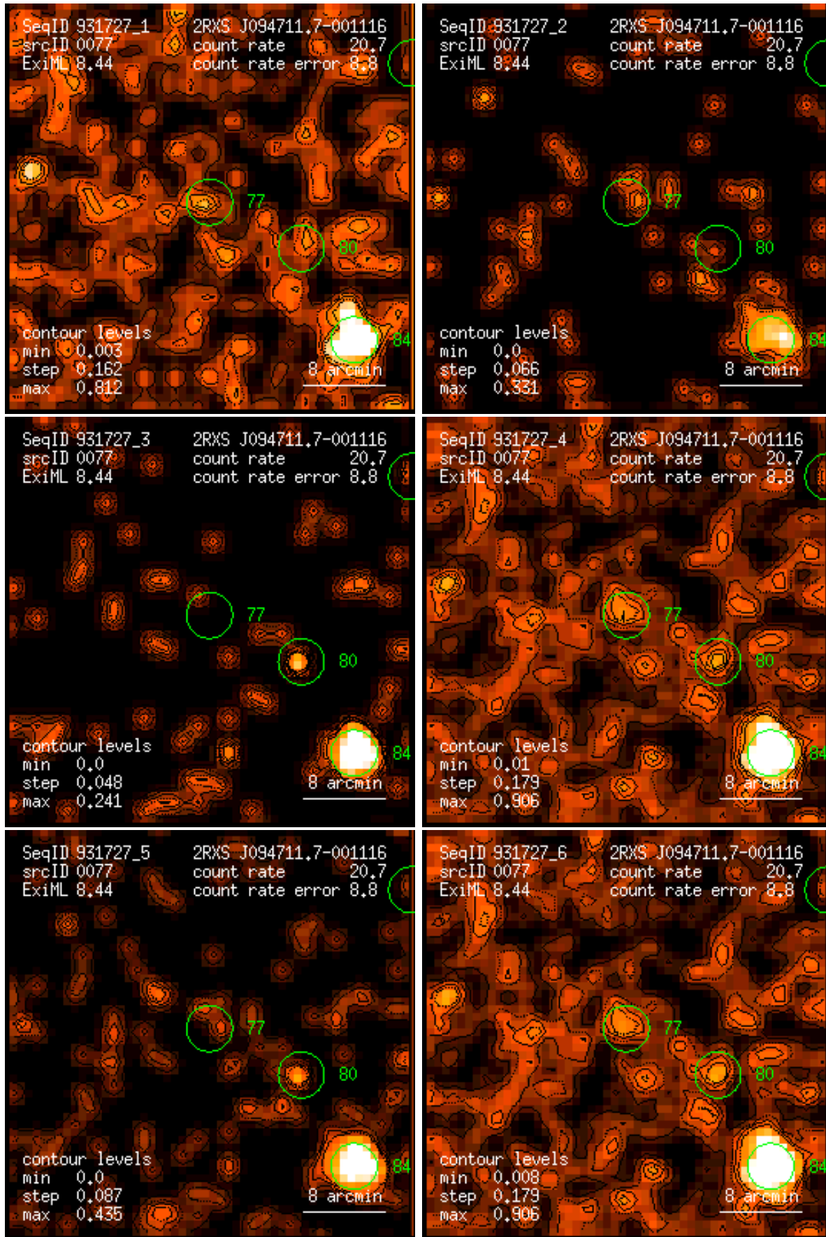
Figure 77: RASS 931727: detection 0077: band rate images, Gaussian filter: (1) PSPP channels 11 – 41, (2) 52 – 90, (3) 91 – 201, (4) 11 – 235, (5) 52 – 201, (6) 11 – 201. Broad band rates in counts/ks. Band rate contour levels in counts/ks/arcmin 2 .
