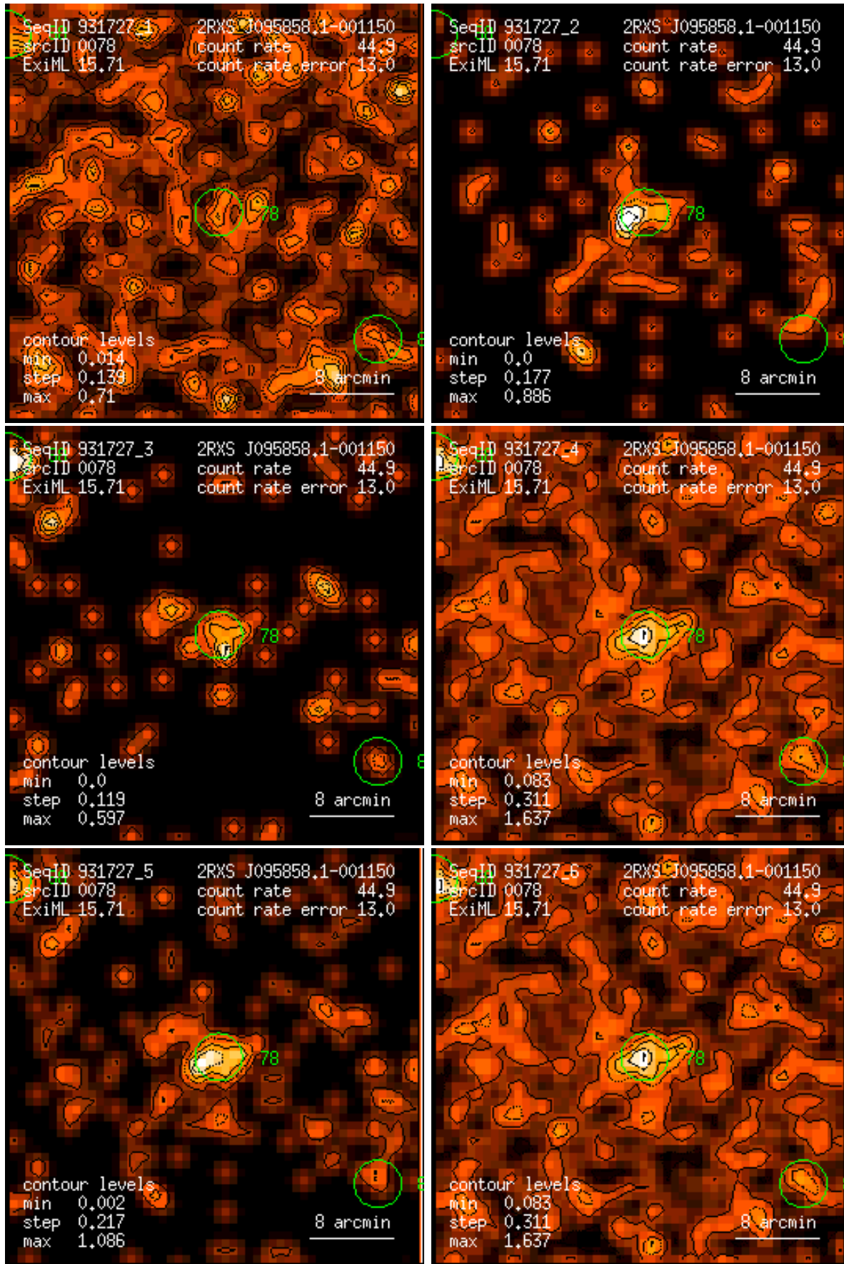
Figure 78: RASS 931727: detection 0078: band rate images, Gaussian filter: (1) PSPC channels 11 – 41, (2) 52 – 90, (3) 91 – 201, (4) 11 – 235, (5) 52 – 201, (6) 11 – 201. Broad band rates in counts/ks. Band rate contour levels in counts/ks/arcmin 2 .
