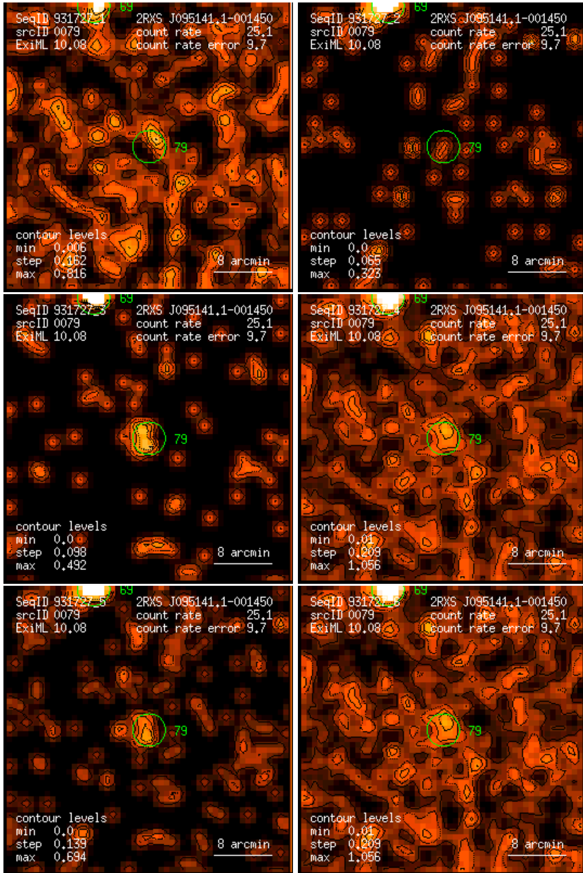
Figure 79: RASS 931727: detection 0079: band rate images, Gaussian filter: (1) PSPC channels 11 – 41, (2) 52 – 90, (3) 91 – 201, (4) 11 – 235, (5) 52 – 201, (6) 11 – 201. Broad band rates in counts/ks. Band rate contour levels in counts/ks/arcmin 2 .
