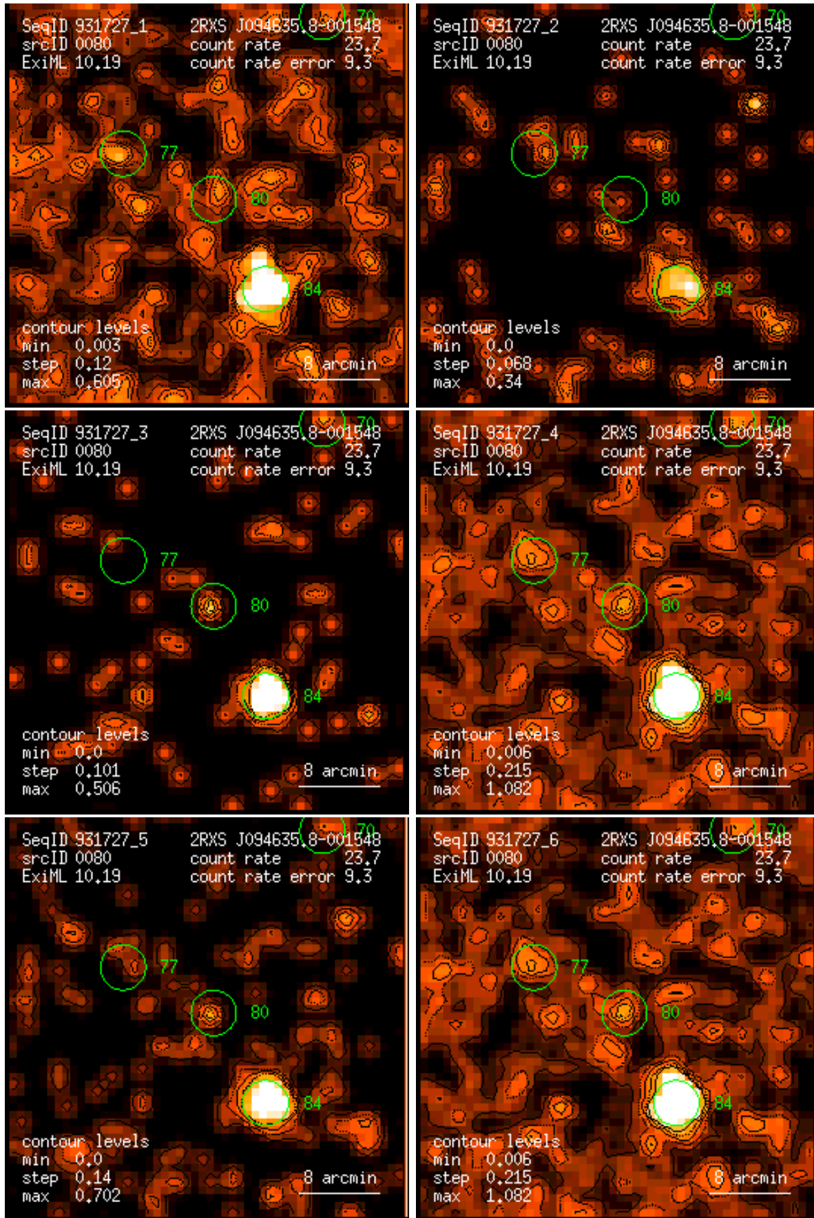
Figure 80: RASS 931727: detection 0080: band rate images, Gaussian filter: (1) PSPC channels 11 – 41, (2) 52 – 90, (3) 91 – 201, (4) 11 – 235, (5) 52 – 201, (6) 11 – 201. Broad band rates in counts/ks. Band rate contour levels in counts/ks/arcmin 2 .
