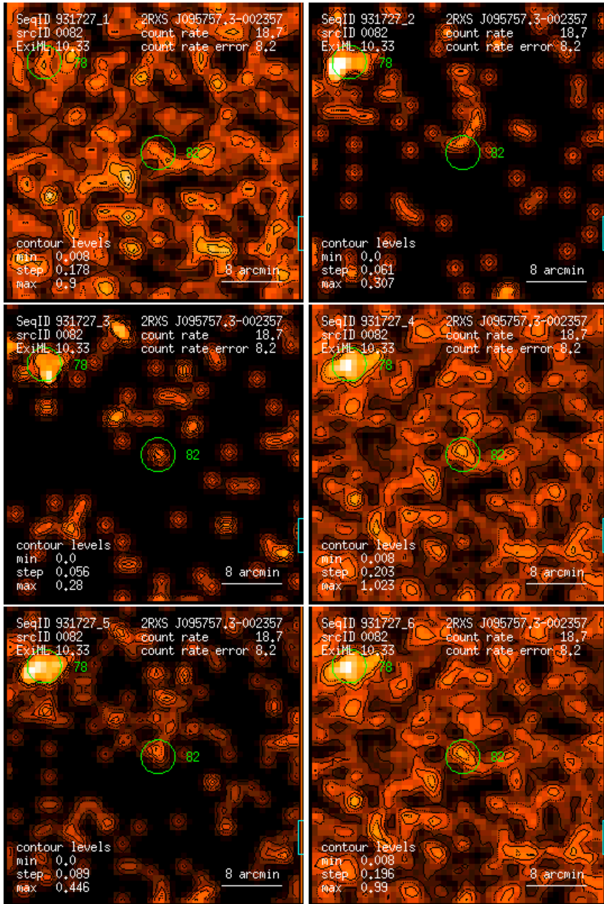
Figure 82: RASS 931727: detection 0082: band rate images, Gaussian filter: (1) PSPC channels 11 – 41, (2) 52 – 90, (3) 91 – 201, (4) 11 – 235, (5) 52 – 201, (6) 11 – 201. Broad band rates in counts/ks. Band rate contour levels in counts/ks/arcmin 2 .
